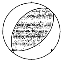
Fig. 11. CMT solution of the mainshock (after Student Group for Realtime Seismology, Earthquake Research Institute, University of Tokyo, 1993; personal communication).
