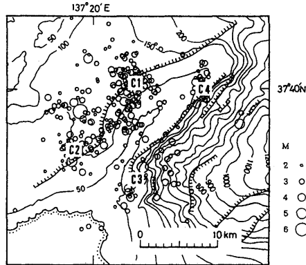
Fig. 8. Clusters of aftershocks. Same as in Fig. 2.
