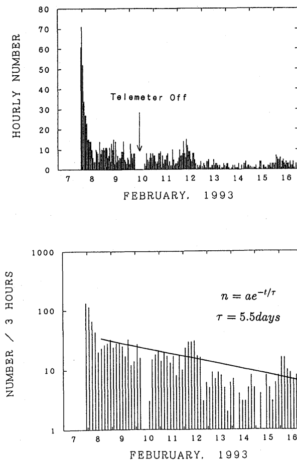
Fig. 14. Time variation of frequency of aftershocks detected at HGR.
