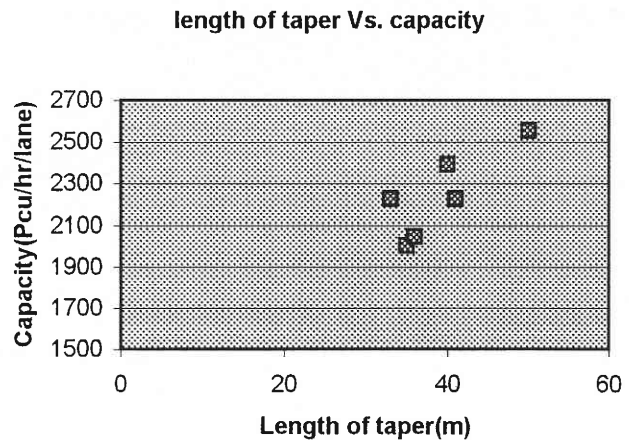
Fig. 2 Relationship between taper length and merging capacity.
