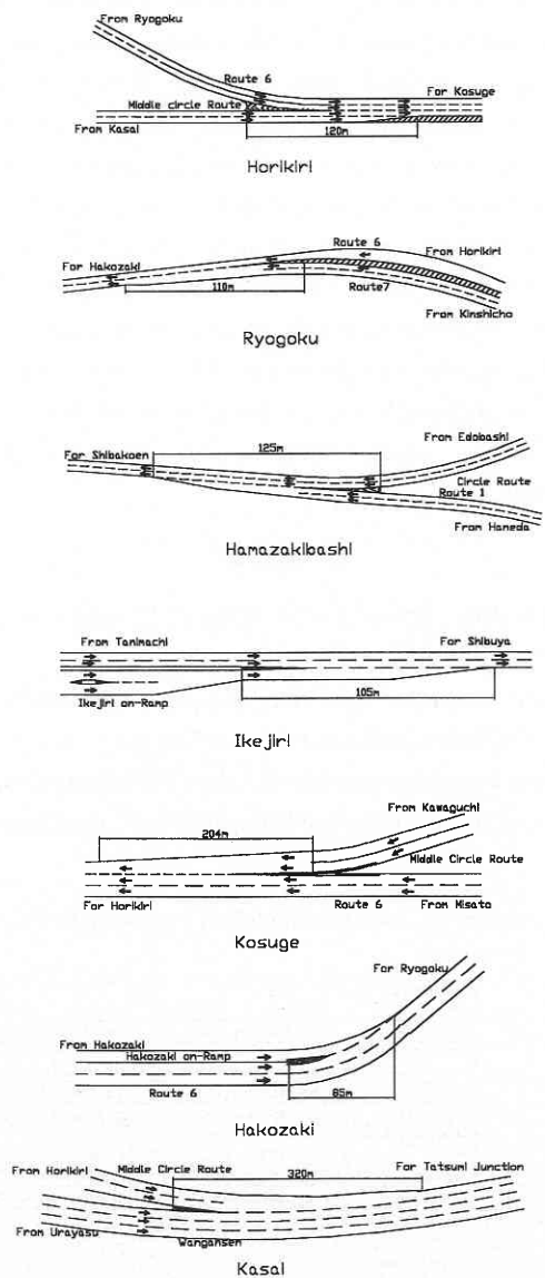
Fig. 1 Tokyo Metropolitan Expressway Merging Segments.
