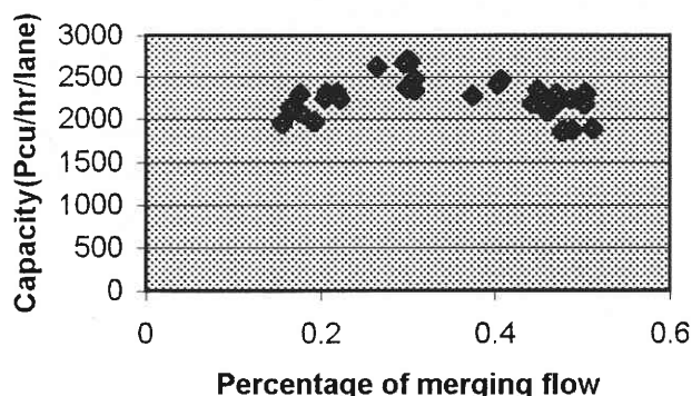
Fig. 5 Relationship between merging ratio and merging capacity.
