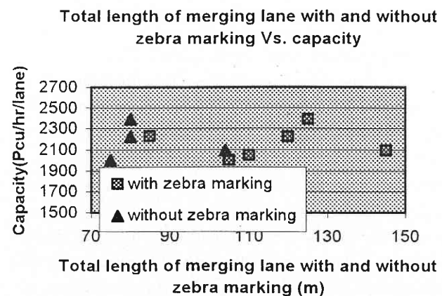
Fig. 3 Relationship between Total length of merging lane with and without zebra marking and merging capacity.
