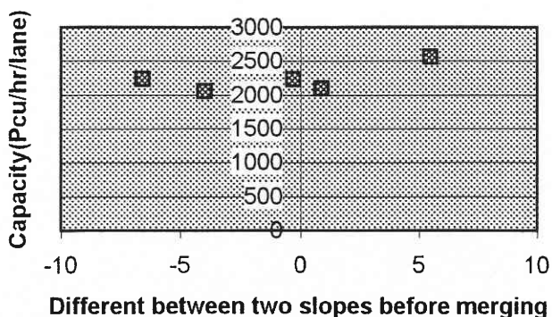
Fig. 4 Relationship between relative slope and merging capacity.
