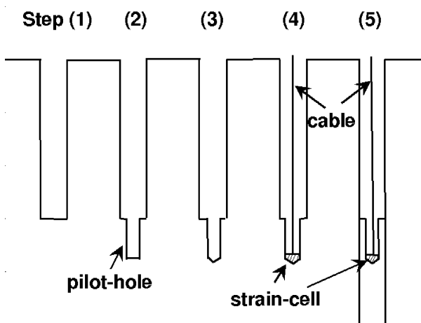
Fig. 1. General procedure of over-coring method. In step 1, a borehole is drilled to the depth of the measurement position with a scale of over-core size. In step 2, a pilot hole is drilled, and in step 3, the bottom of the pilot hole is ground to a semi-spherical or conical shape for borehole bottom measurement. In step 4, a strain-cell is embedded inside the borehole or glued to the bottom. In step 5, the pilot hole is over-cored.
