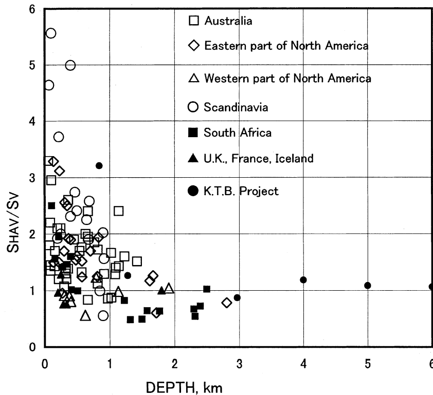
Fig. 8. Ratio between mean horizontal stress ( S_{HAV}=(S_H+S_h)/2 ) and overburden stress ( S_v ) increases ground surface approaches. Based on the figure of Brown and Hoek [1978], KTB result [Brudy et al. , 1997] is added. In the original figure, data for North America were classified in two groups, data in Canada and those in the U.S.A. In this figure, the data for North America are classified into data for the eastern and western parts of the North American continent.
