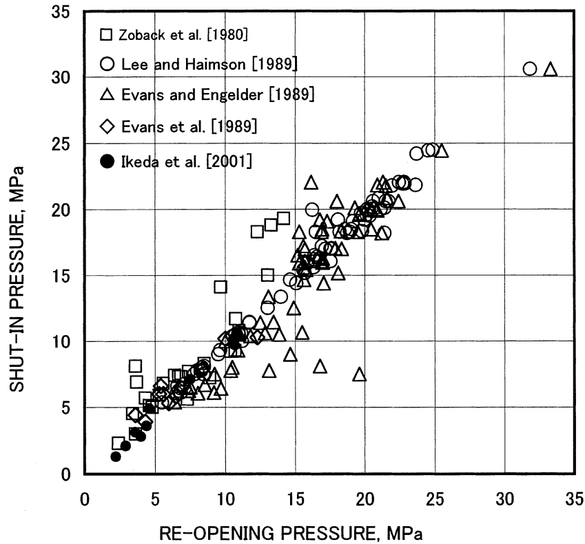
Fig. 4. An example of the relationship between the re-opening pressure ( P_r ) and the shut-in pressure ( P_s ) obtained in the U.S.A., Canada, and Japan. Many results indicate the relationship, P_r = P_s , which suspiciously shows that (S_H + P_p) / S_h is equal to 2.0 at any depth around the world.
