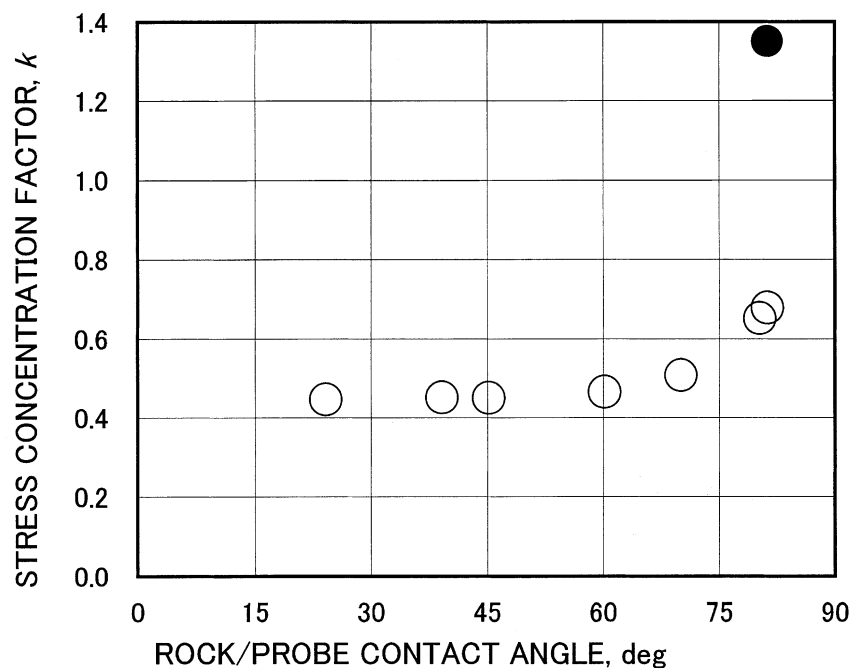
Fig. 7. For the newly designed borehole-jack stress probe, the stress distribution on the borehole wall is influenced by the elastic coupling of the probe/borehole contact. The stress concentration factor defined by ratio, hoop stress at the mouth of the fracture, and jack pressure, is plotted against the rock/probe close contact angle. The results shown by open circles indicate the stress concentration factor for the continuous coupling from the left-hand edge to the right-hand edge through the apex of the outer shell (see Fig. 6c). The result shown in the solid circle shows the result assuming a very thin space around the apex of the shell. The solid circle indicates the highly effective loading condition. However, the concentration factor might fall to almost half of the solid circle, if the coupling conditions are not the same as designed conditions. Hence, we may use the coupling conditions as shown in solid circle only in the fracturing process, but we have to use the coupling conditions shown by open circles for the re-opening procedures.
