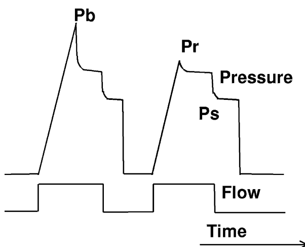
Fig. 3. Schematic of hydrofracturing procedure. The borehole is pressurized at a constant flow rate. When fractures are formed, a sudden pressure drop is always observed. The peak pressure is called the breakdown pressure ( P_b ). The fractures extend at a constant flow rate. When the valve for flowing water is closed, the pressure decreases to a constant level called the shut-in pressure ( P_s ). P_s is known to be equal to the stress component normal to the fracture. After complete closure of the fractures, the borehole is pressurized again to re-open the fractures. Several re-loading cycles are performed in conventional hydraulic fracturing procedures as shown in Fig. 5.
