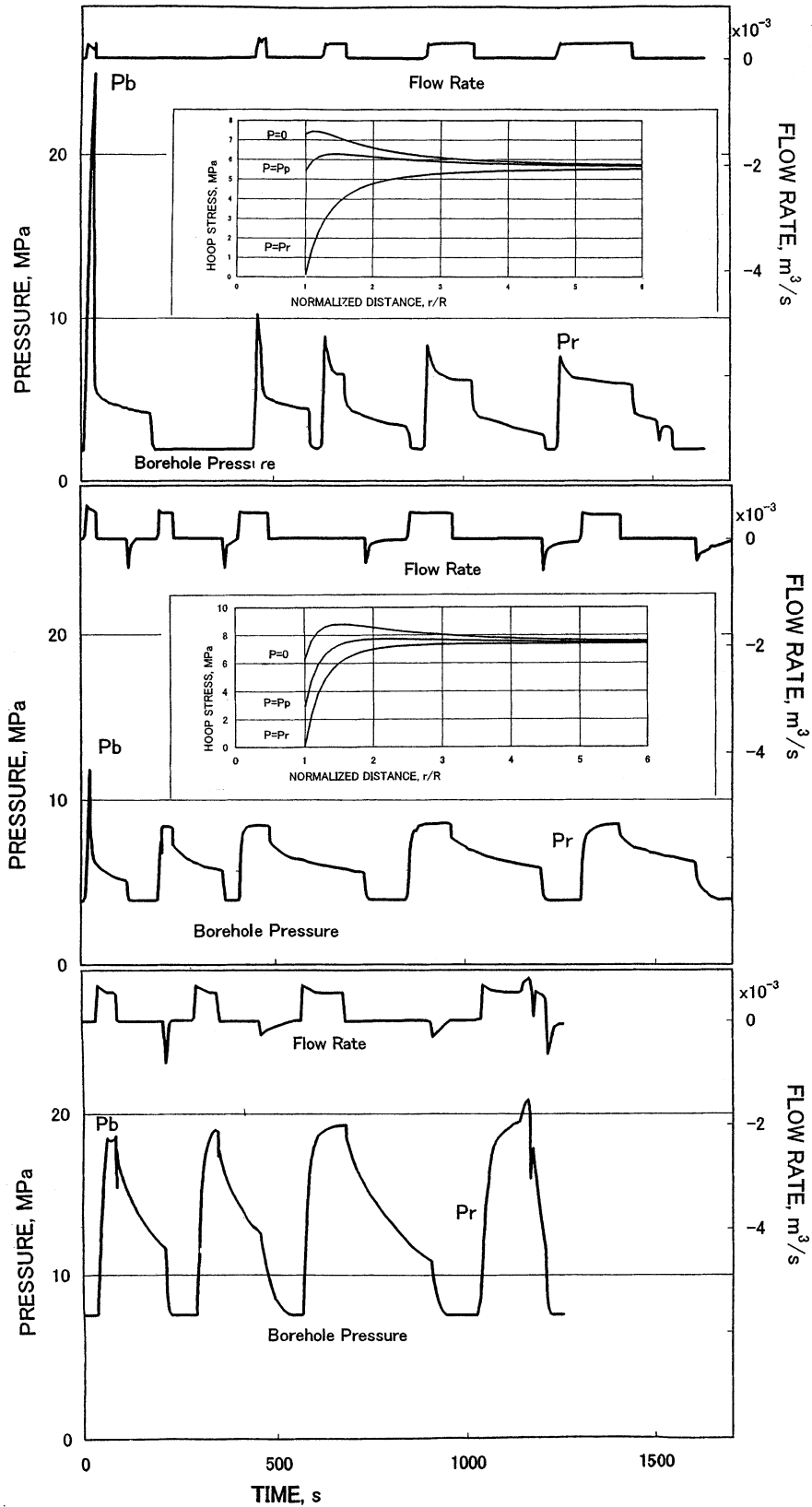
Fig. 5. Typical pressure/time curves of hydraulic fracturing tests. The figures after Hickman and Zoback [1982] are modified by adding hydrostatic pressure to borehole pressure. (a), (b), and (c) correspond to the results at depths of 185 m, 338 m, and 751 m, respectively. In each figure, the flow rate and the borehole pressure are shown at upper and lower sides, respectively. In (d) and (e), calculated hoop stress is plotted against distance from borehole axis.
