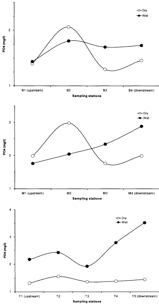
Fig. 4. PO 4 3- values for 3 rivers in Manado City, SB (a), SM (b), and ST (c) during dry and wet seasons. Stations are shown on Fig. 1.
