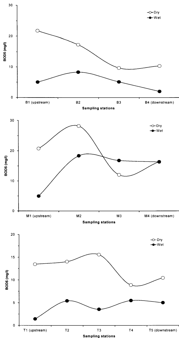
Fig. 2. BOD 5 values for 3 rivers in Manado City, SB (a), SM (b), and ST (c) during dry and wet seasons. Stations are shown on Fig. 1.
