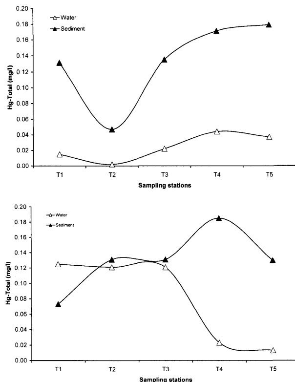
Fig. 6. Concentration of Hg-tot in water and sediment of ST during dry (a) and wet (b) seasons. Stations are shown on Fig. 1.
