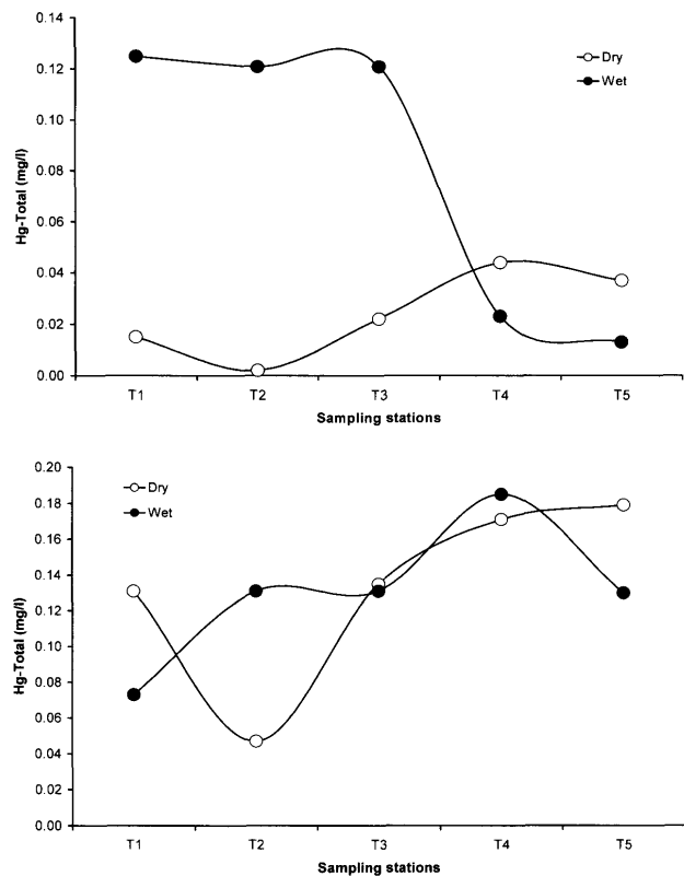
Fig. 5. Concentration of Hg-tot in water (a) and sediment (b) of ST during dry and wet seasons. Stations are shown on Fig. 1.
