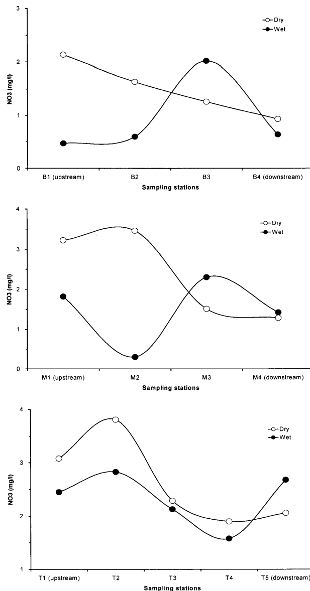
Fig. 3. \text{NO}_3^- values for 3 rivers in Manado City, SB (a), SM (b), and ST (c) during dry and wet seasons. Stations are shown on Fig. 1.
