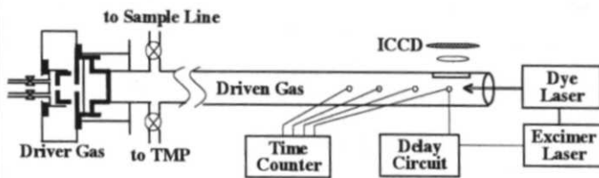
Fig.1 Experimental apparatus.
