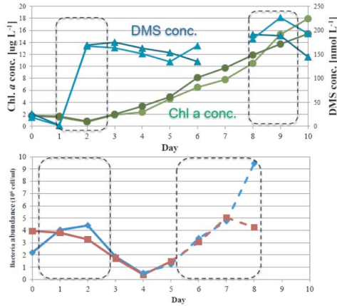
Fig. 2-2a. DMS and chl-a concentration and bacterial abundance during a coccolithophorid bloom.
