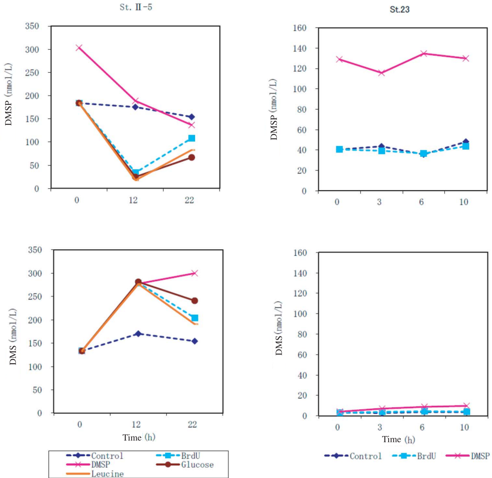
Fig. 1-4. DMS and DMSP concentrations at St. 23.
