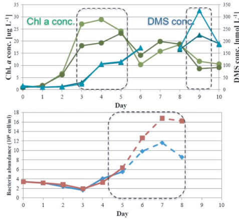
Fig. 2-1a. DMS and chl-a concentration and bacterial abundance during a diatom bloom.
