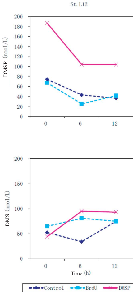
Fig. 1-1. DMS and DMSP concentrations at St. L12.
