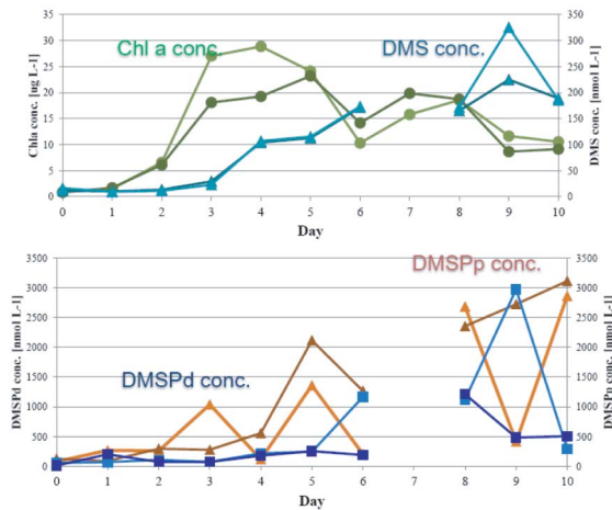
Fig. 2-1b. DMS, DMSP and chl-a concentration during a diatom bloom.
