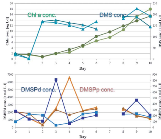
Fig. 2-2b. DMS, DMSP and chl-a concentration during a coccolithophorid bloom.
