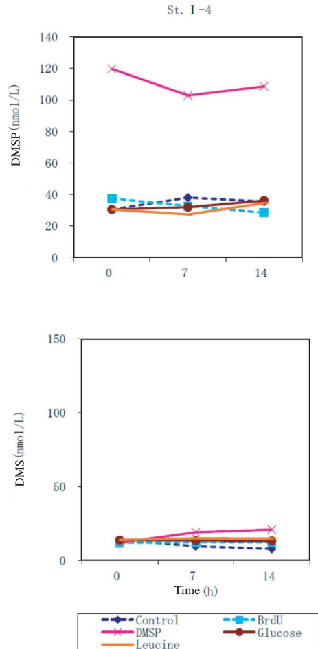
Fig. 1-2. DMS and DMSP concentrations at St. I-4.
