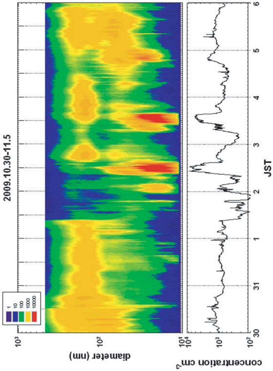
Fig. 2. Size distributions measured at Cape Ochiishi, between 30 Oct. and 5 Nov., 2009.
