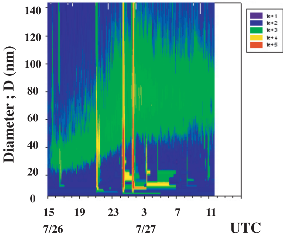
Fig. 1. Size distributions measured on R/V Hakuho Maru, on 26 and 27 July, 2004.
