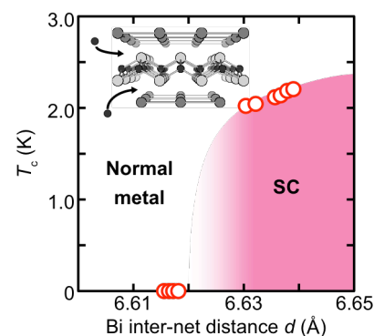
Figure 4. Superconducting phase diagram of \text{Y}_2\text{O}_2\text{Bi} as a function of d . Inset shows schematic image of O incorporation. SC: superconducting.
