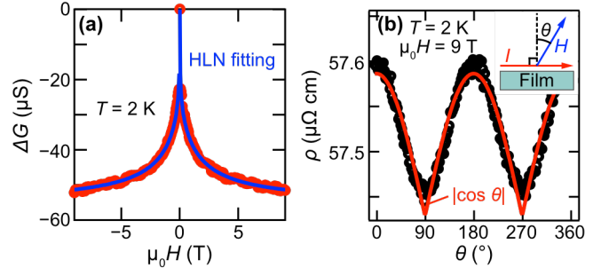
Figure 2. (a) Magnetoconductance at 2 K and (b) angular dependent magnetoresistance at 2 K and 9 T of Y_2O_2Bi epitaxial thin film. Inset of (b) denotes measurement configuration.
