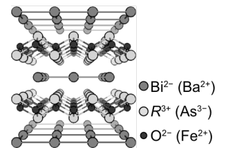
Figure 1. Crystal structure of R_2O_2Bi .
