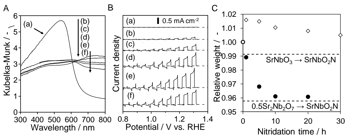
Figure 1. (A) DR spectra, (B) current-potential curves, and (C) relative weight of SrNbO 2 N nitrided from SrNbO 3 for various nitridation time. (a) oxide precursor, (b) 1 h, (c) 5 h, (d) 10 h, (e) 20 h, (f) 30 h. In (C), relative weight of SrNbO 2 N nitrided from Sr 2 Nb 2 O 7 for various nitridation time are also shown for comparison (●).
