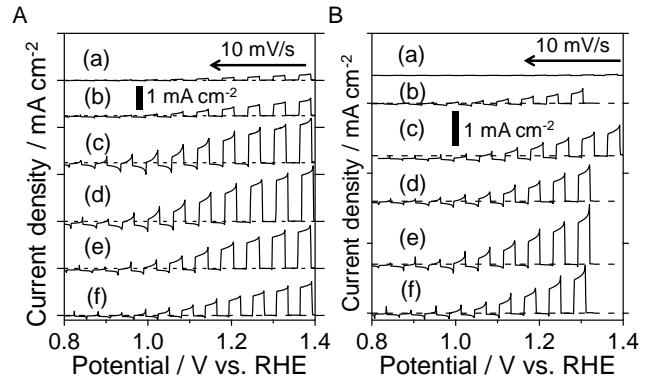
Figure 3. Current-potential curves of CoPi/SrNbO 2 N/Nb/Ti photoanodes nitrided from (A) NaSrNbO with various nitridation time. (a) 0.02, (b) 1, (c) 3, (d) 7.5, (e) 10 and (f) 15 h. (B) Current-potential curves of CoPi/SrNbO 2 N/Nb/Ti photoanodes nitrided from Sr 2 Nb 2 O 7 with various nitridation time. (a) 0.02, (b) 1, (c) 3, (d) 5, (e) 10 and (f) 20 h. The PEC measurements were performed under AM 1.5G irradiation in 0.2 M Na 3 PO 4 (pH adjusted to 13 by NaOH addition).
