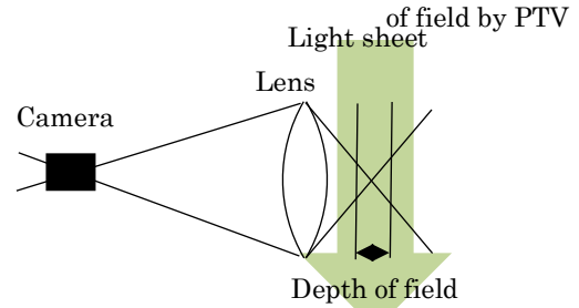
Fig.7 Relationship between light sheet and depth of field by PTV
