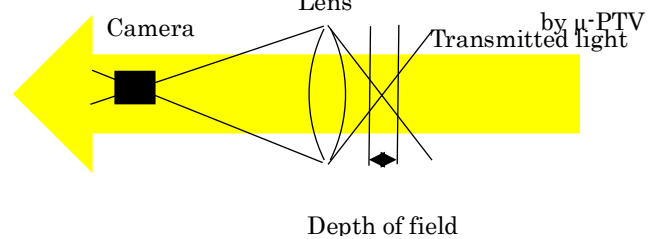
Fig.8 Relationship between transmitted light and depth of field by μ-PTV
