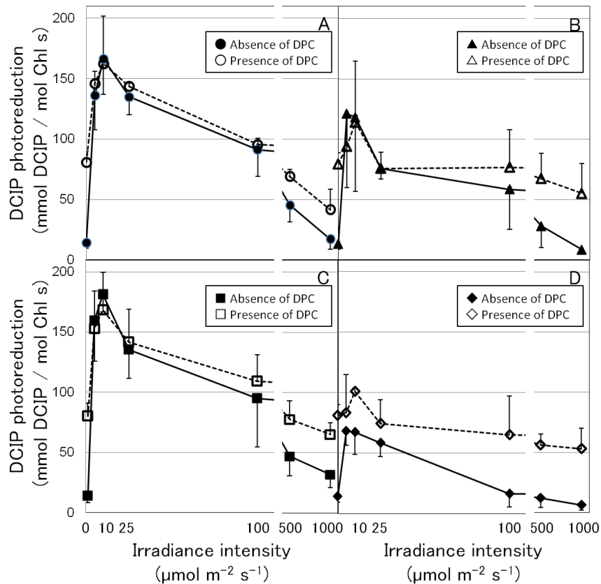
Fig. 2 DCIP photoreduction rates in the absence and presence of DPC of the thylakoid membranes after reactivation treatment.
