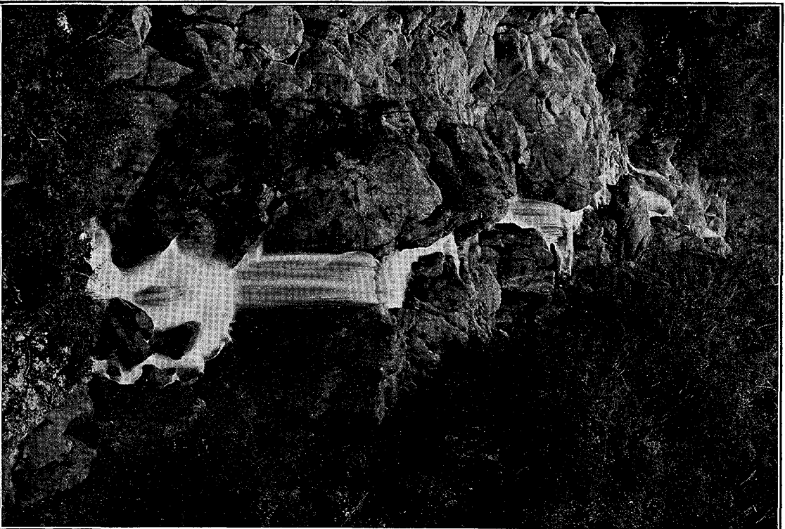
Fig. 1. Chigo-otoshi waterfall.
