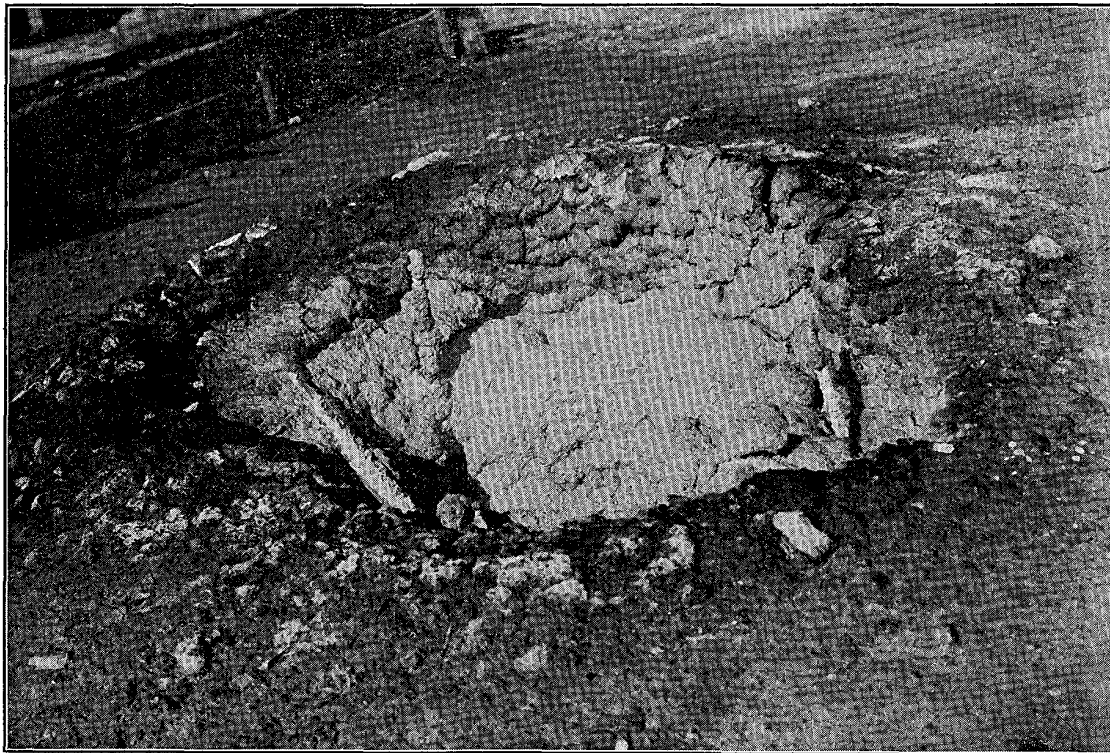
Fig. 2. The mud volcano in Shinyu.
