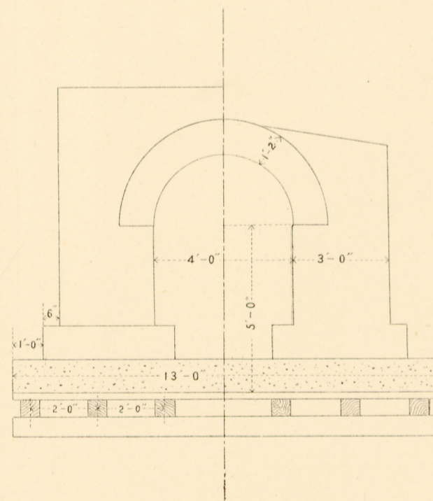
CROSS SECTION.
