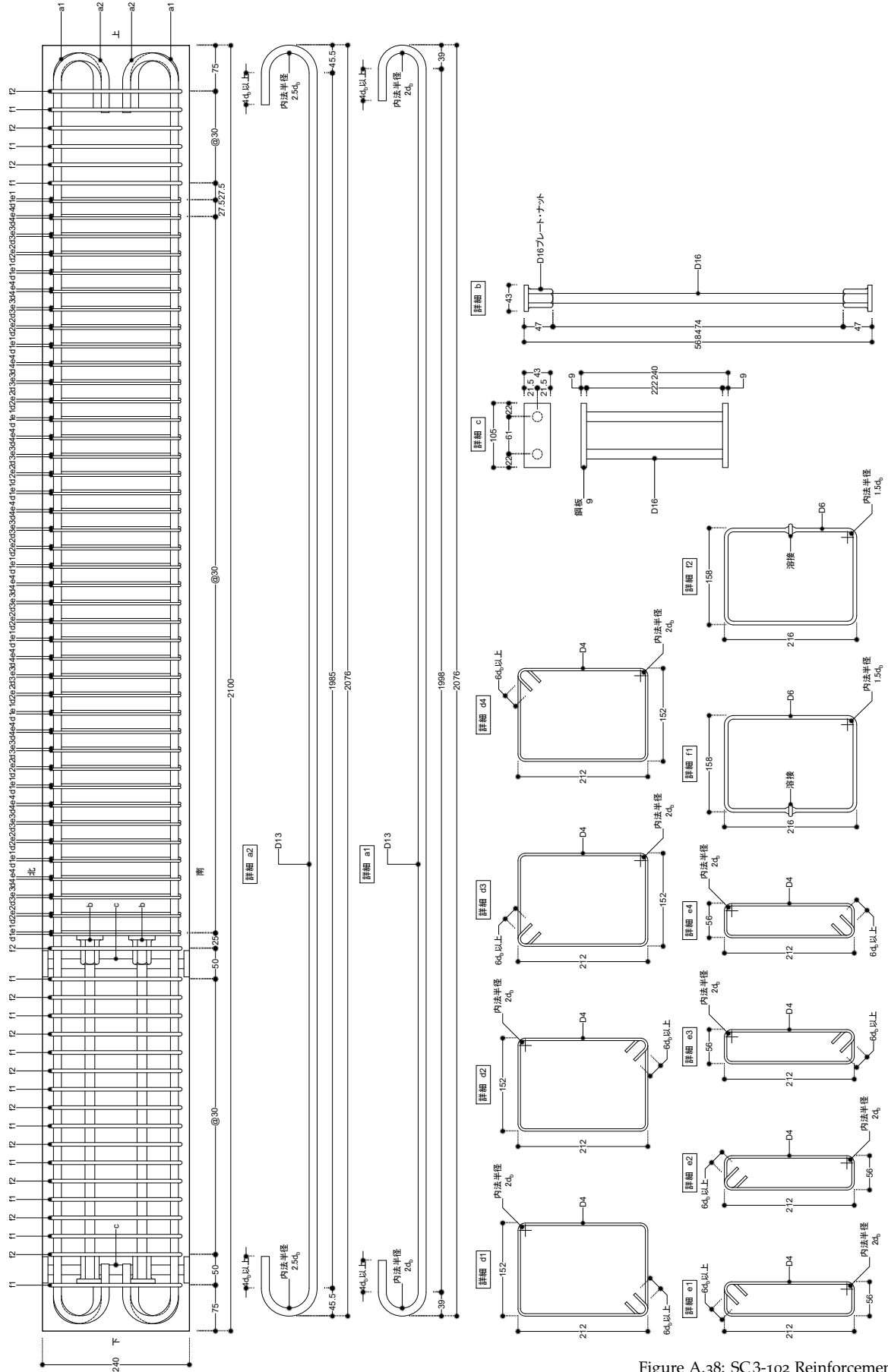
Figure A.38: SC3-102 Reinforcement details
