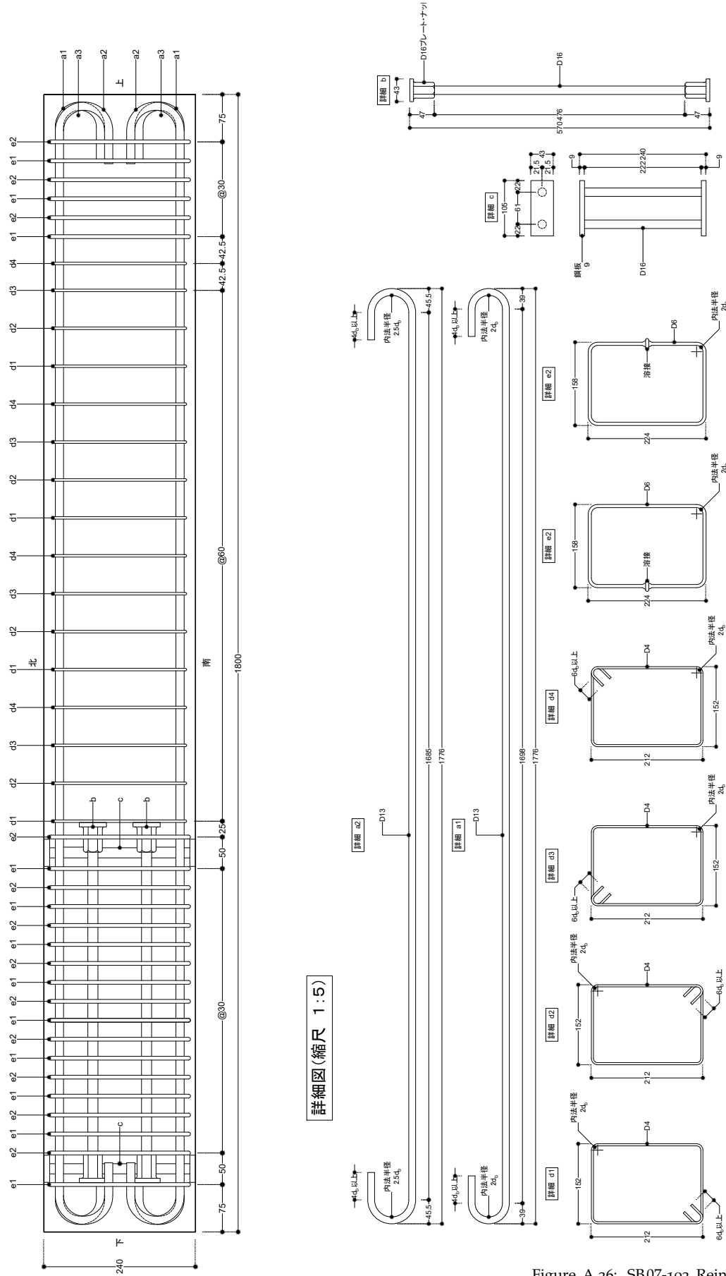
Figure A.26: SB07-102 Reinforcement details
