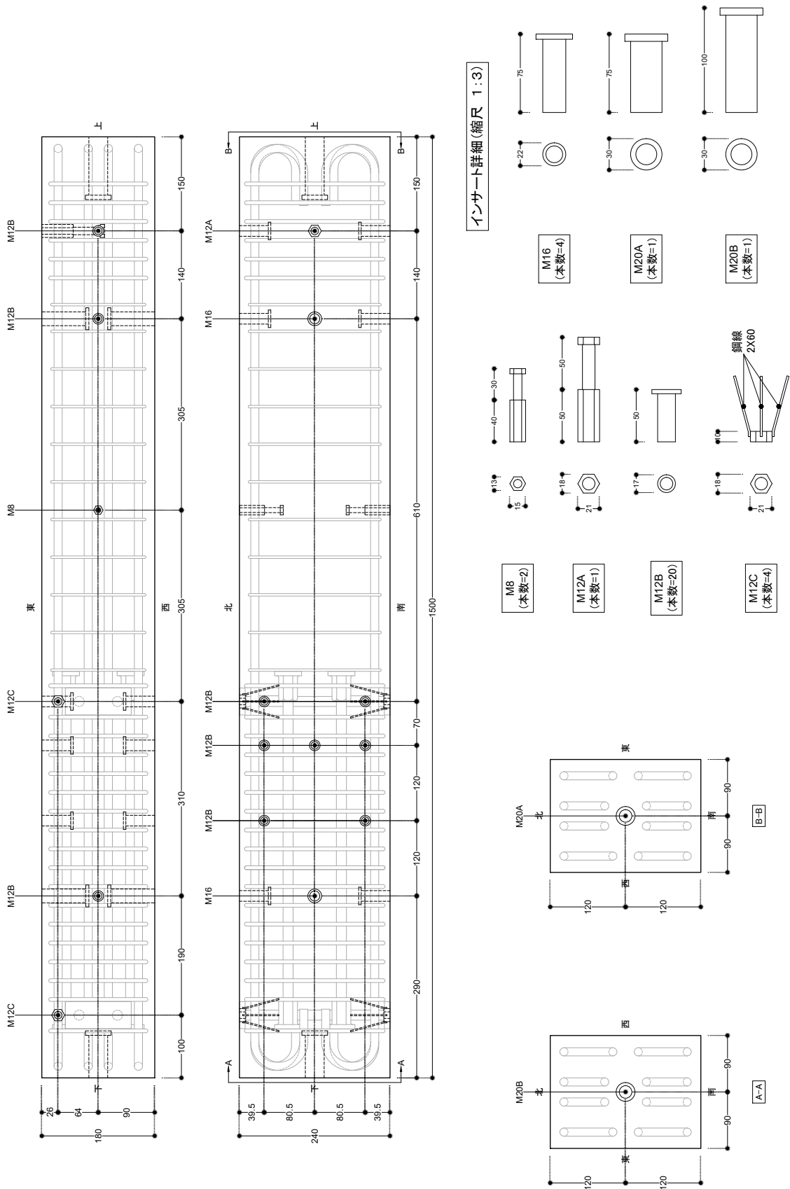
Figure A.16: SB01-104 Insert arrangement
