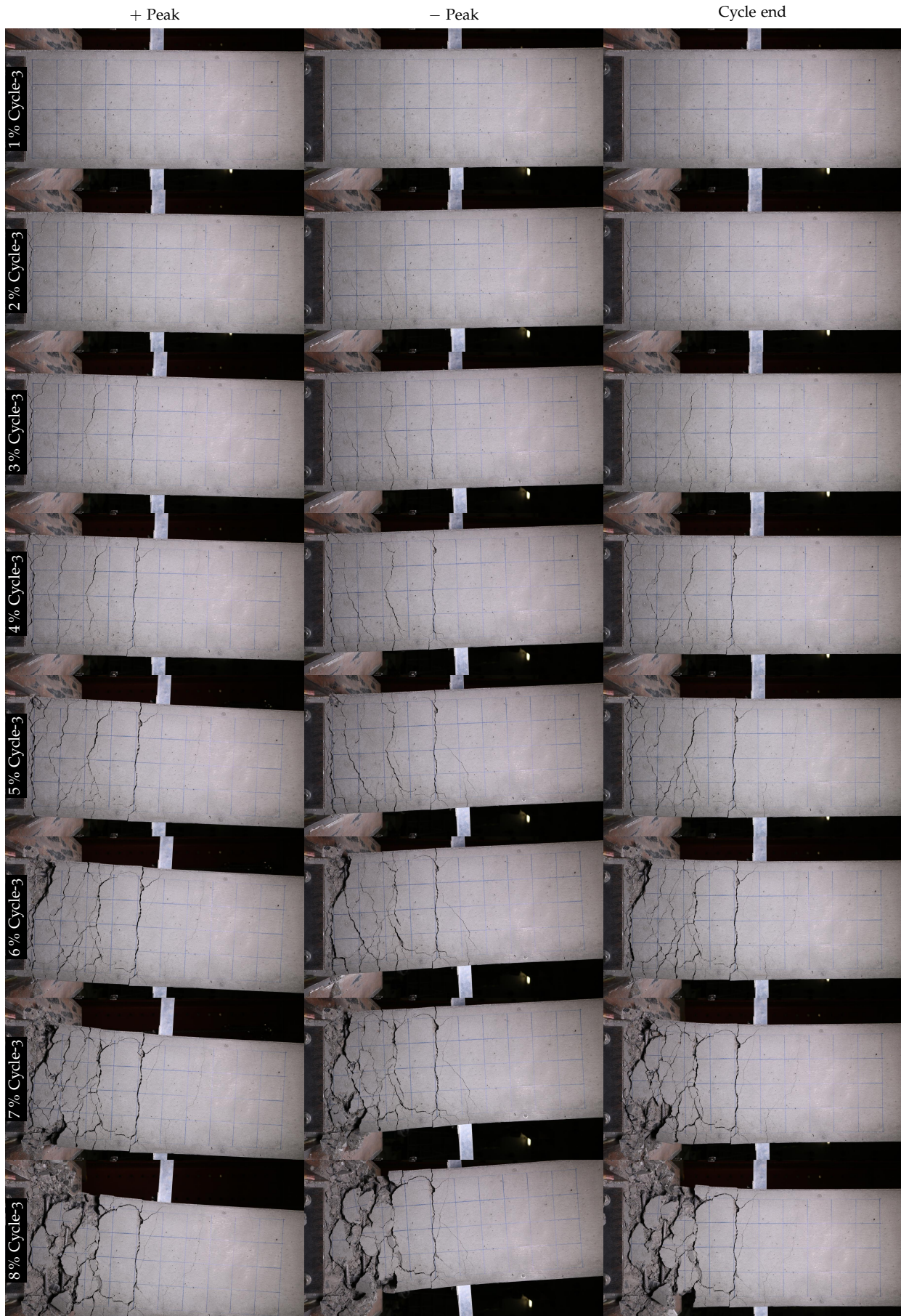
Figure D.19: Damage states at peak and cycle completion loading states (SC4)
