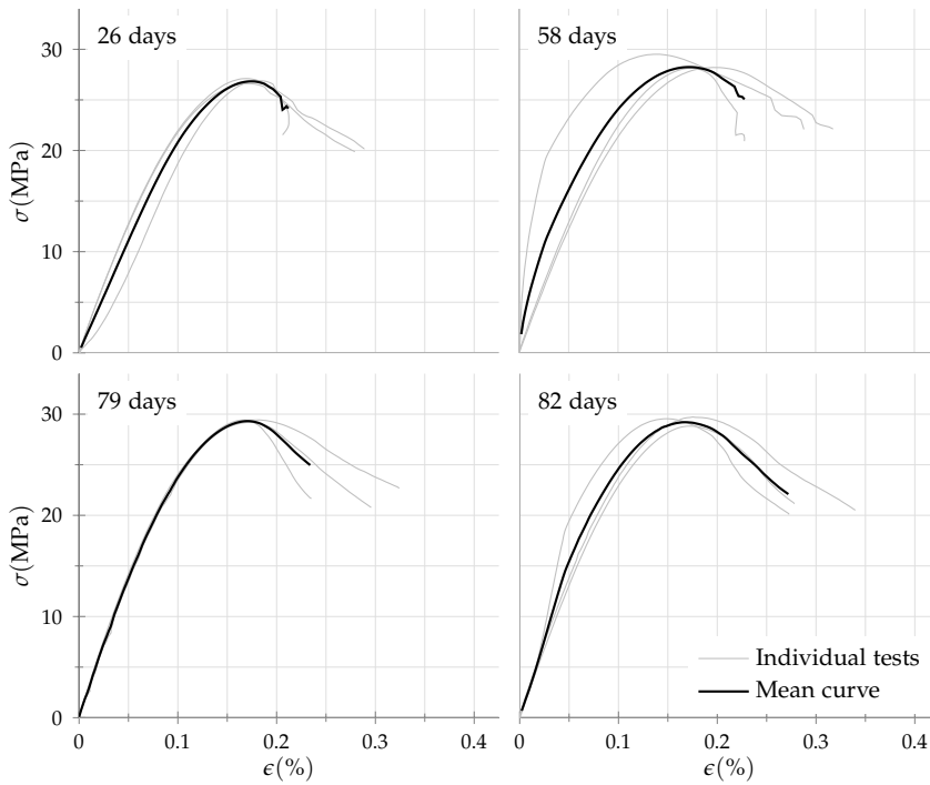
Figure B.2: Concrete material test results for SA batch
