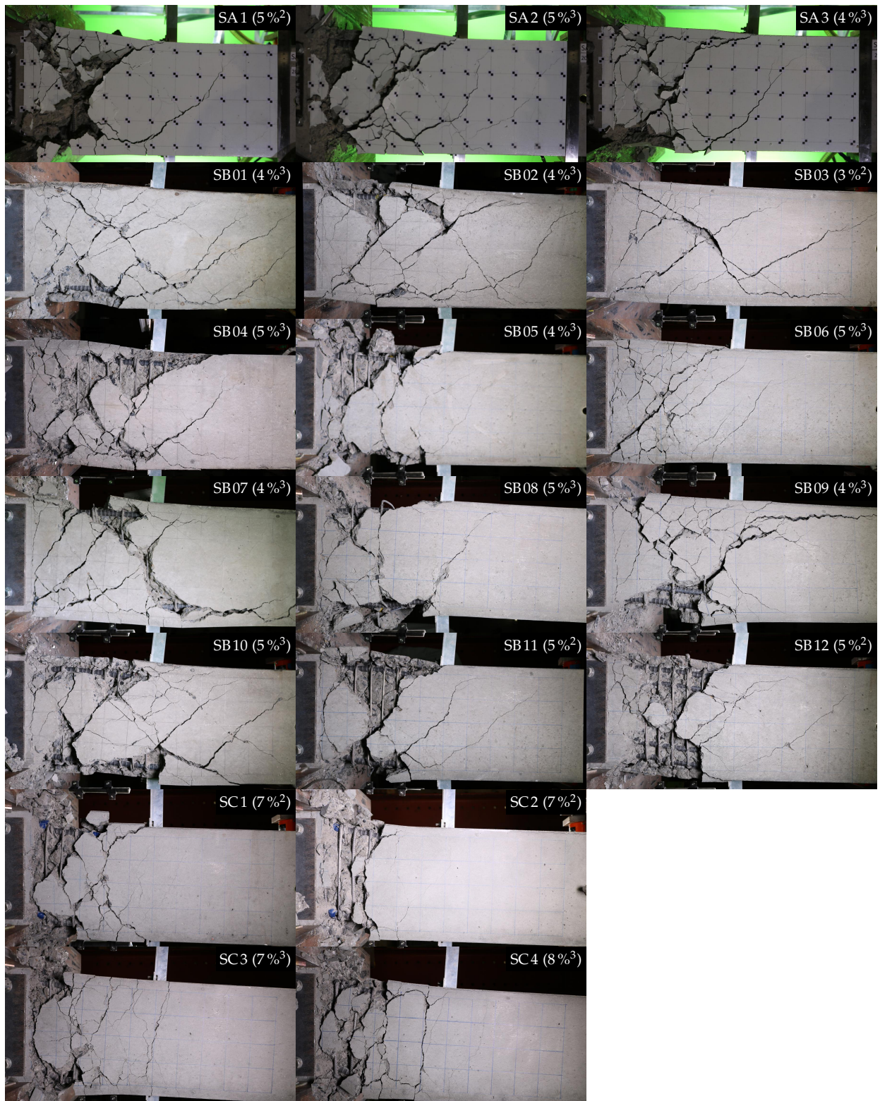
Figure 4.4: Comparison of damage states for all specimens at loss of resistance state
