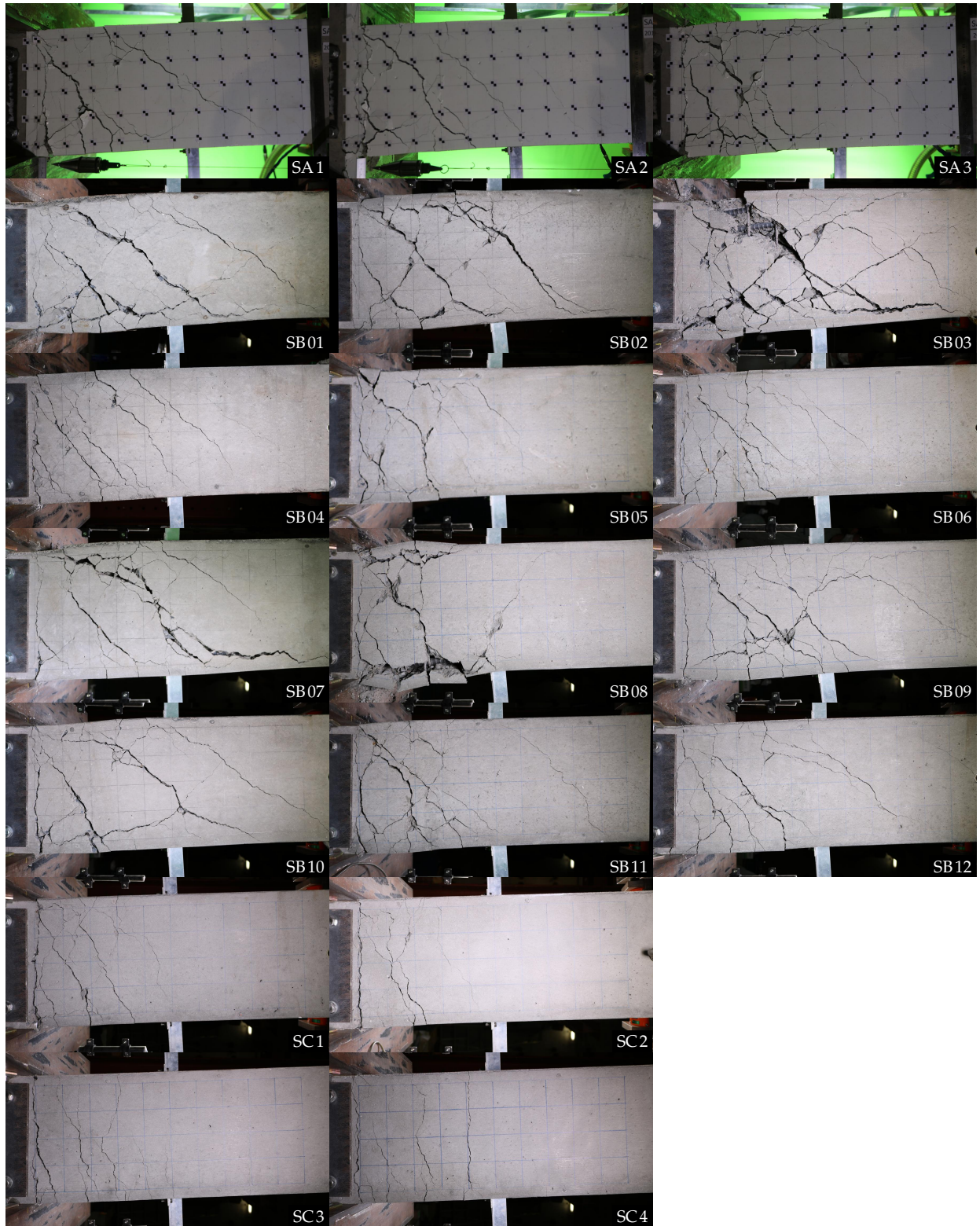
Figure 4.2: Comparison of damage states for all specimens at peak of first loading cycle at -4% target drift
