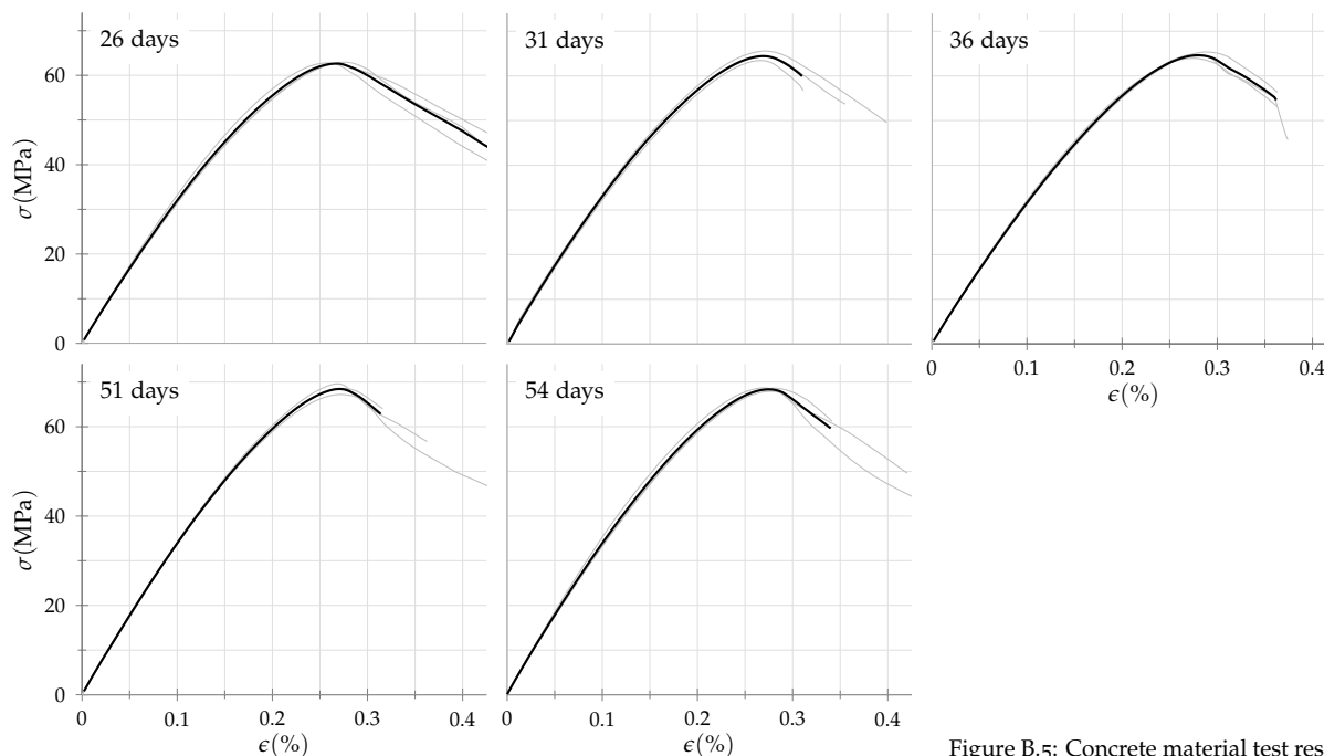
Figure B.5: Concrete material test results for SC batch Table B.8: SA batch concrete test results at 58 days
