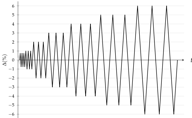
Figure 3.16: Applied loading history
