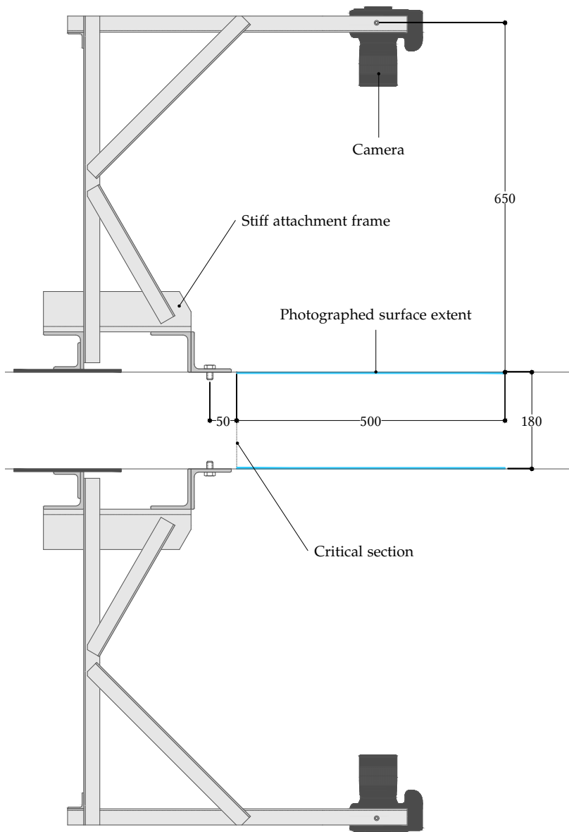
Figure 3.13: Frame for camera positioning (all dimensions are in mm)
