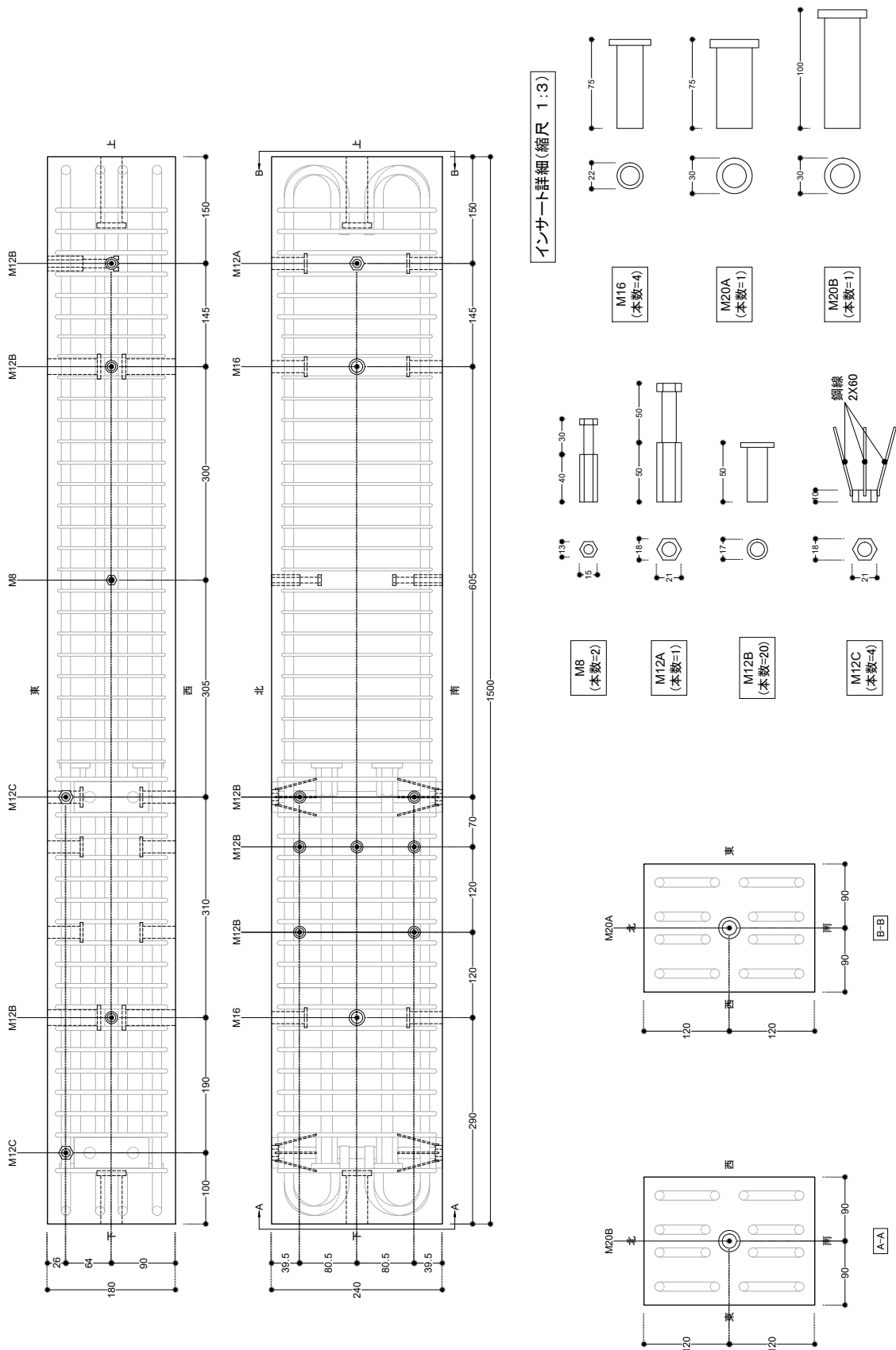
Figure A.24: SB04-104 Insert arrangement
