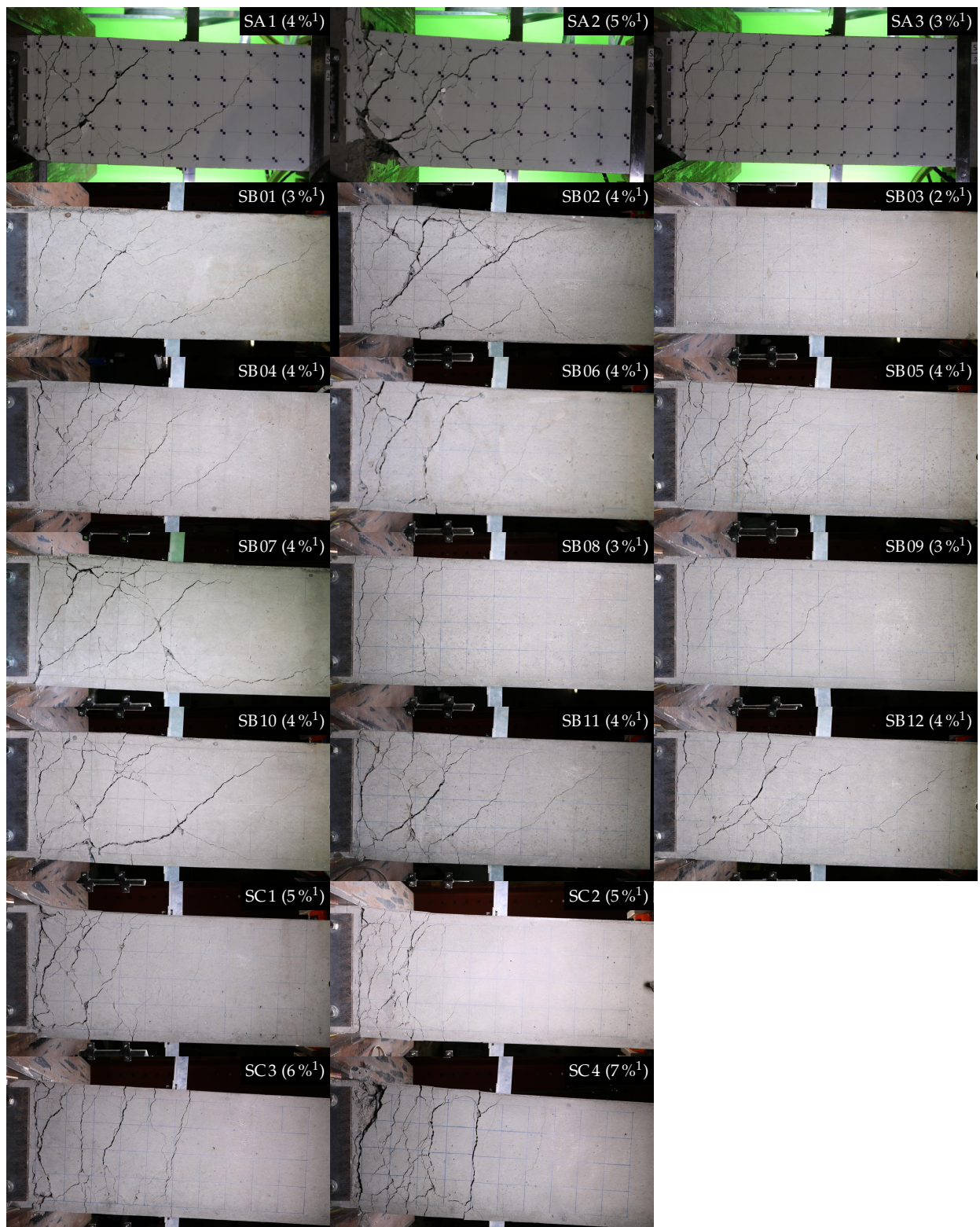
Figure 4.3: Comparison of damage states for all specimens at peak resistance state
