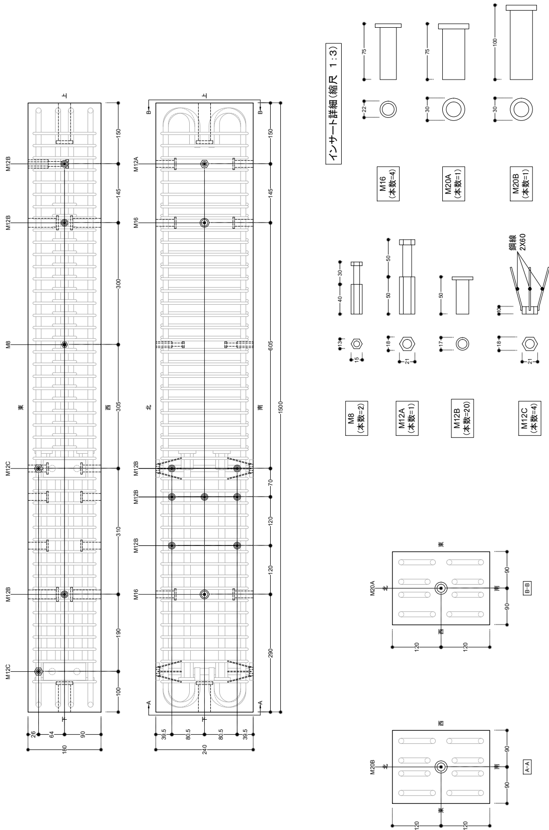
Figure A.36: SC2-104 Insert arrangement
