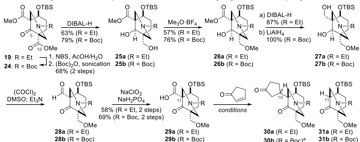
Scheme 5. Preparation of carboxylic acid 29 , and its radical coupling reaction with cyclopentenone
