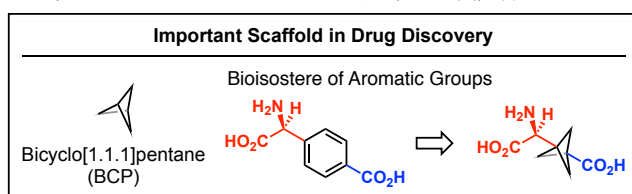
Figure 1. Bicyclo[1.1.1]pentane.
