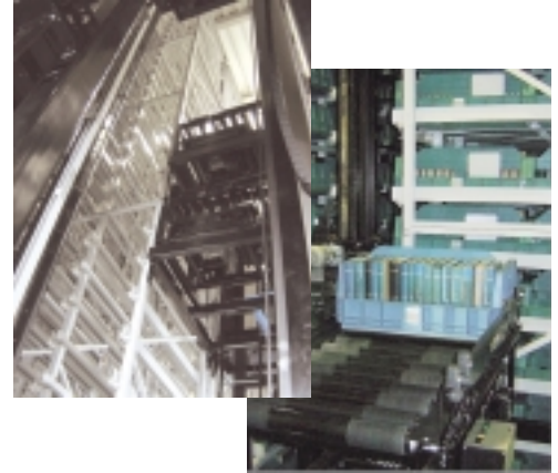
Kashiwa Library-ASRS (Automated Storage and Retrieval System)
