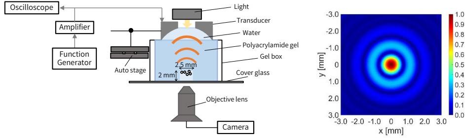
Fig. 1 (Left): Experimental setup, (Right): Pressure distribution on the focal plane
