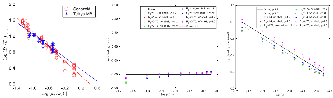
Fig.2 (Left): Relation between diameter of bubble clouds and incident ultrasound frequency, (Center): Relation between scaling factor and void fraction in the bubble cloud, (Right): Relation between coefficient and void fraction in the bubble cloud
