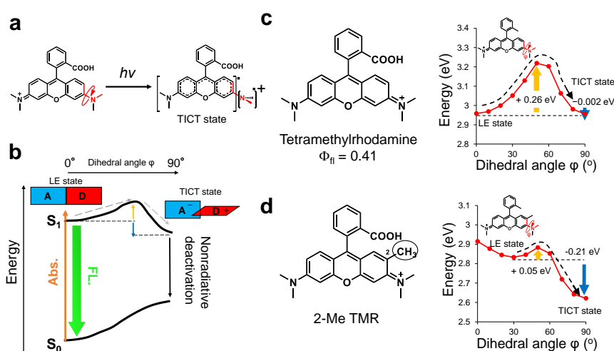
Figure 1. (a) TICT formation of tetramethylrhodamine. (b) Schematic illustration of energy dependences of S_0 and S_1 states of rhodamine dyes on dihedral angle ( \phi ). A: acceptor. D: donor. (c,d) Energy dependences of S_1 states of tetramethylrhodamine (c) and 2-Me TMR (d) on dihedral angle ( \phi ). Geometries of conformers were optimized at CAM-B3LYP/6-31G+(d,p) level.
