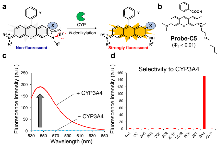
Figure 3. (a) Design strategy of a fluorescent probe for N -dealkylation activity of CYPs. (b) Chemical structure and \Phi_{fl} of Probe-C5. (c) Fluorescence spectral change of Probe-C5 (1 \mu M) before and 30 min after addition of CYP3A4 (10 nM) (Ex. 520 nm). (d) Fluorescence intensity of Probe-C5 (1 \mu M) 10 min after addition of various CYP enzymes (5 nM) (Ex. 520 nm, Em. 550 nm). Assays were performed in the presence of NADPH generating system.
