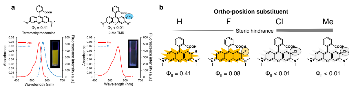
Figure 2. (a) Photophysical properties, absorption and emission spectra of 1 \mu M tetramethylrhodamine (left) and 2-Me TMR (right) measured in PBS (pH 7.4). (b) \Phi_f of rhodamine dyes with different substituents at the 2 position of the xanthene moiety.
