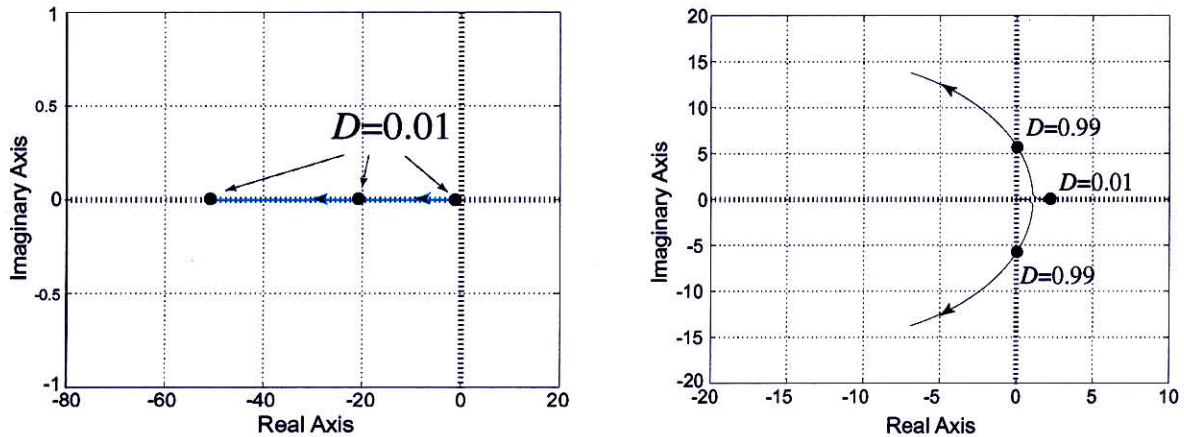
(a) 慣性変動なし ( J_n = J, M = 0.3 )
