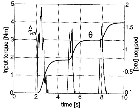
(b) M = 1.0 , D = 3.0
