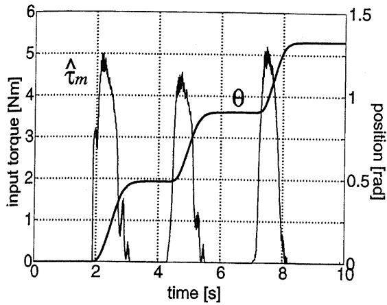
(a) M = 1.0 , D = 7.0
