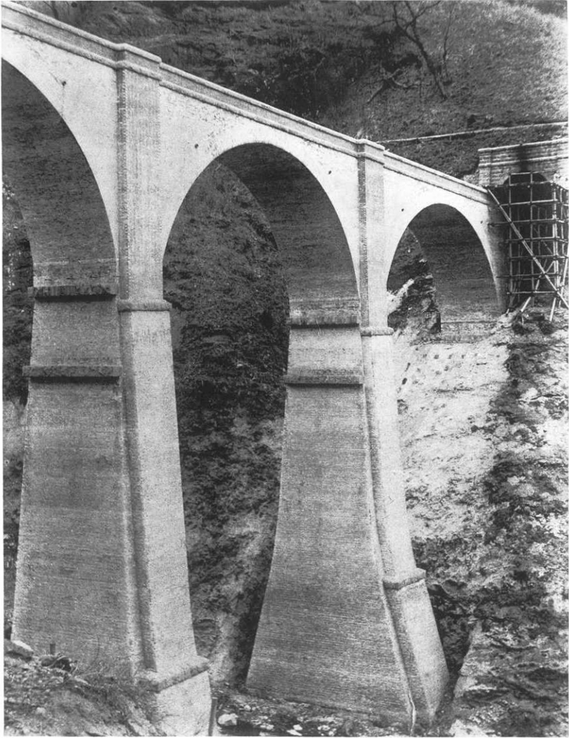
PARABOLIC PIERS ON THE USUI PASS (110 FEET HIGH).
