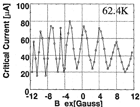
Fig. 2. The magnetic modulation of the critical current at 62.4 K for the junction 5 \mu\text{m} wide and 300 nm thick
