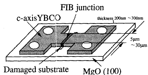
Fig. 1. Schematic illustration of YBaCuO co-planar Josephson junction using FIB
