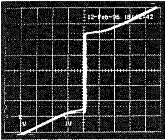
Fig. 4. The I-V characteristic of the junction 200 nm thick and 10 \mu\text{m} wide at 4.8 K. x-axis: 50 \mu\text{V}/\text{div} ; y-axis: 0.2 mA/div
