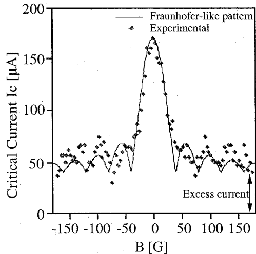
Fig. 7. The magnetic field modulation of the critical current for the junction of 7 \mu\text{m} width and 200 nm thickness at 4.2 K.
