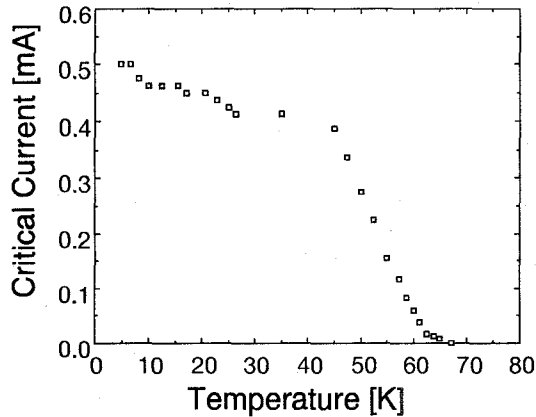
Fig. 5. The temperature dependence of the critical current of the junction. The junction is the same as in Fig.4.
