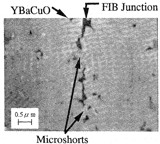
Fig. 3. The surface of the FIB junction by SEM photograph; Microshorts were observed on the junction.
