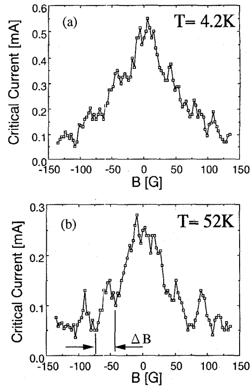
Fig. 6. The magnetic field modulation of the critical current for the junction of 10 \mu\text{m} width and 200 nm thickness at (a) 4.2 K and (b) 52 K.
