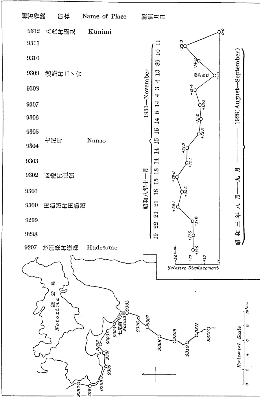
第 1 圖 富山縣水見郡八代村國見より石川縣鹿島郡笠師保村葦染に至る一等水準線檢測圖 (Relative vertical displacements of bench marks along the route from Yatusiro-mura to Kasaiho-mura via Nanao.)
