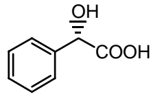
(S)-4
