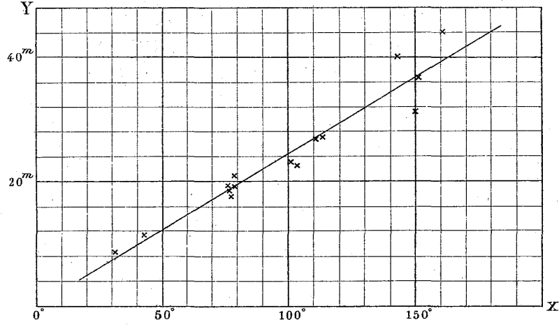
Fig. 2, b. Guatemala earthquake: Curve for P 2 .
