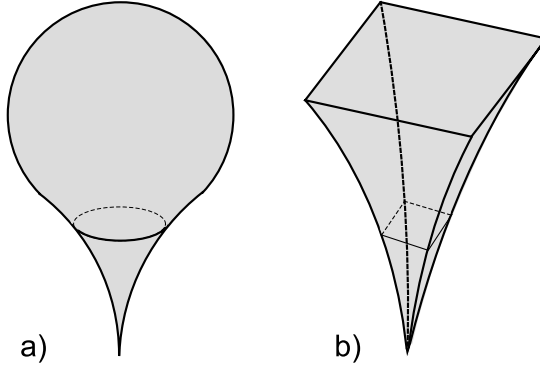
Fig. 1.2. Peak-shaped domains.
