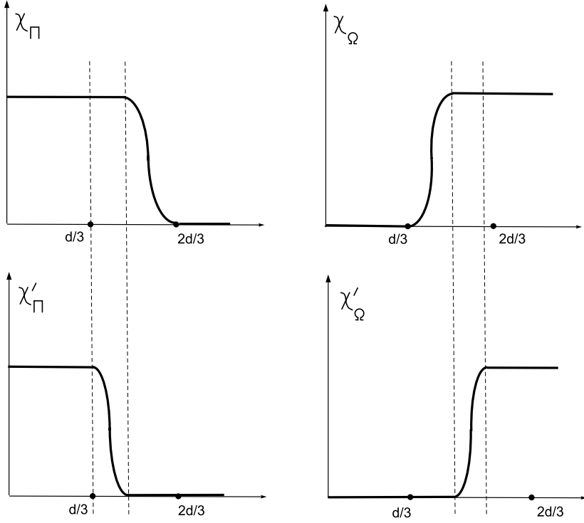
Fig. 2.1. Cut-off functions.
