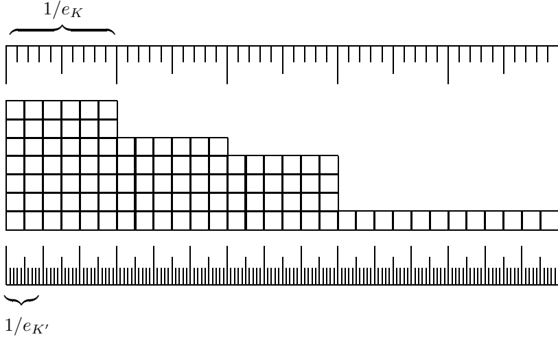
Fig. 1. Rulers graduated in units of sizes 1/e_K , 1/e_{K'}
