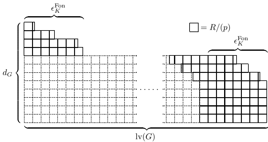
Fig. 5. t_G(K/R) \otimes_R R/(p^{\epsilon_K^{\text{Fon}}+1})
