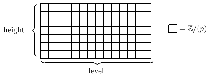
Fig. 2. The group of \overline{K} -valued points of a group scheme of p -rectangle-type
