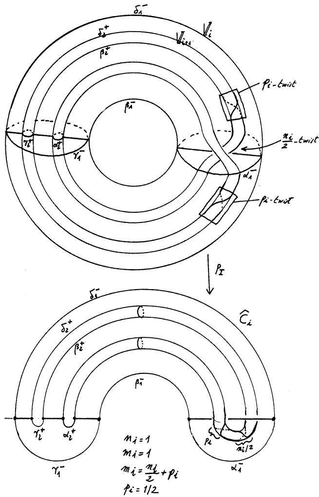
Fig. 14. The restriction of p_I : \mathbb{S}^3 \rightarrow \mathbb{S}^3 to the solid tori pair (V_i, V_{i+1}) .
