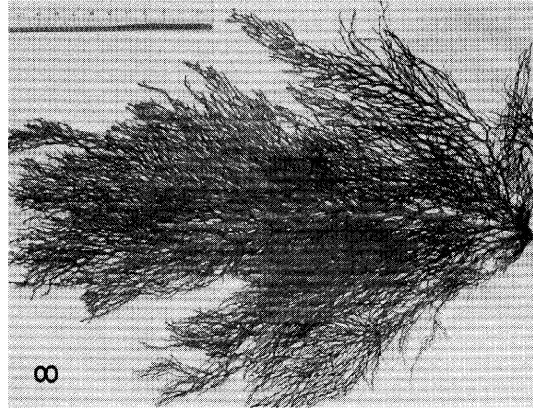
Figs. 5-8. Herbarium specimens of Halymenia from Malaysia. Fig. 5. SAP090439, Fig. 6. SAP090444, Fig. 7. SAP090438, Fig. 8. KWGSH80.
