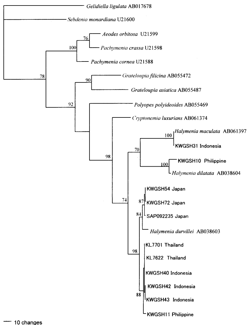
Fig. 30. Maximum parsimony tree for rbcL sequences of 11 Halymenia specimens (with KWGSH, SAP and KL numbers), 10 halymeniacean species and two outgroups downloaded from GenBank (with AB and U numbers).
