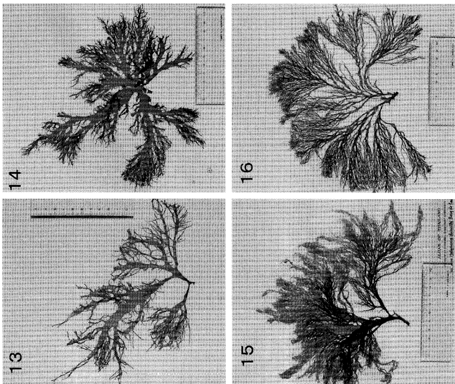
Figs. 13-16. Herbarium specimens of Halymenia from Thailand. Fig. 13. KL7611, Fig. 14. KL7701, Fig. 15. KL7622, Fig. 16. KL7621.
