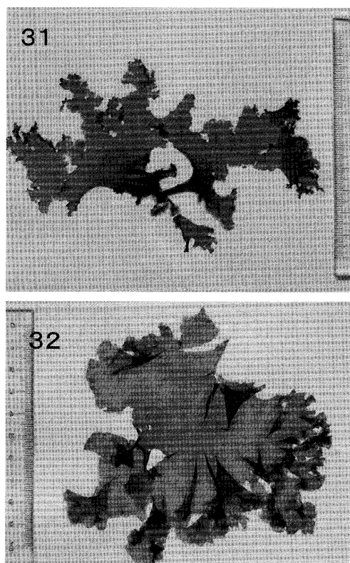
Figs. 31, 32. Herbarium specimens of foliose Halymenia from Indonesia and the Philippines. Fig. 31. KWGSH31, Fig. 32. KWGSH10.
