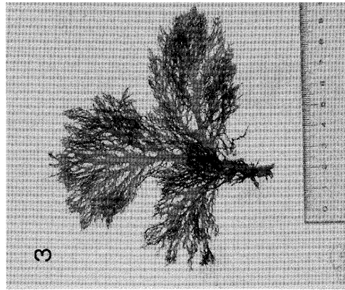
Figs. 1-4. Herbarium specimens of Halymenia from Japan and the Philippines. Fig. 1. KWGSH72 (Japan), Fig. 2. KWGSH54 (Japan), Fig. 3. SAP092235 (Japan), Fig. 4. KWGSH11 (the Philippines).
