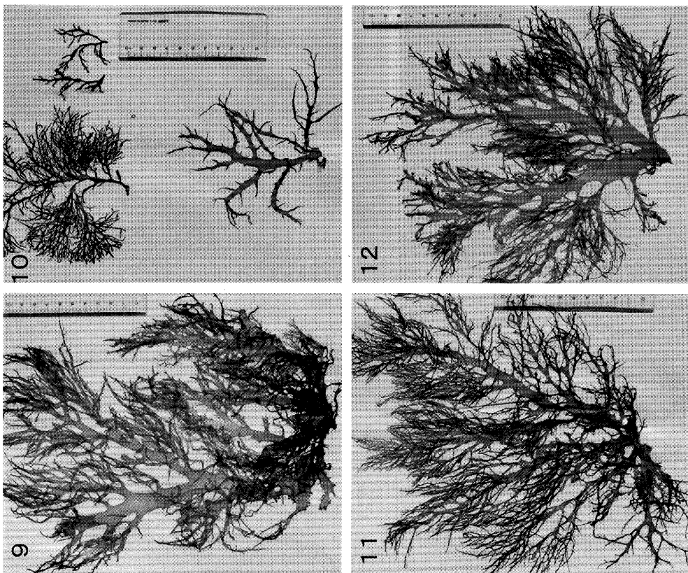
Figs. 9-12. Herbarium specimens of Halymenia from Indonesia. Fig. 9. KWGSH42, Fig. 10. KWGSH40, Fig. 11. KWGSH43, Fig. 12. KWGSH41.
