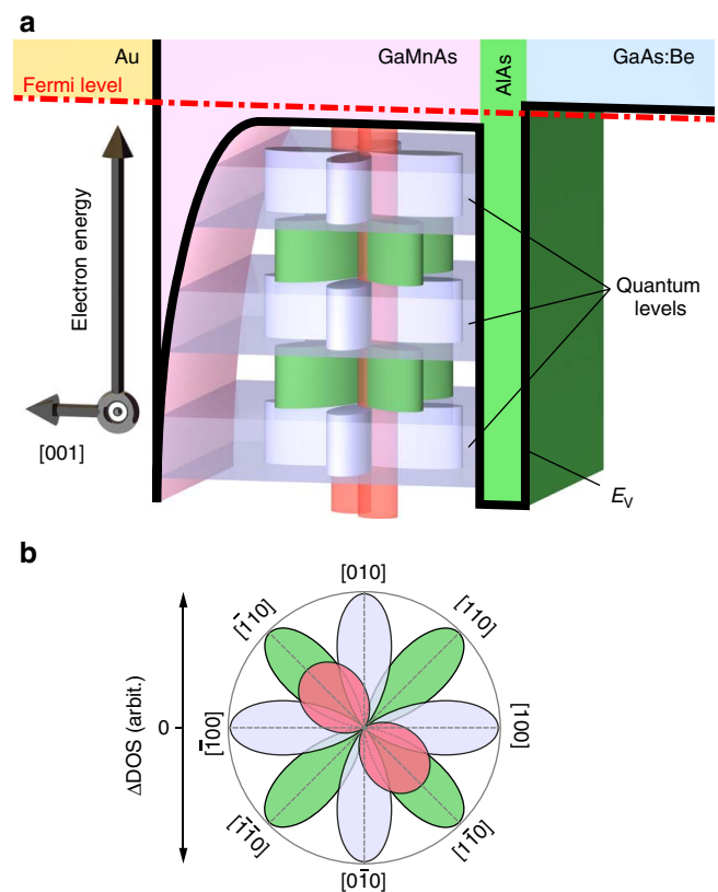
Figure 1 | Schematic valence band diagram representing our findings.
