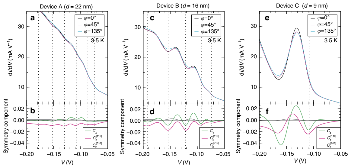
Figure 5 | Relationship between the differential conductance and symmetry components. (a,c,e) The dI/dV - V characteristics measured at \varphi = 0^\circ (black), \varphi = 45^\circ (pink) and \varphi = 135^\circ (light blue) on devices A–C, respectively. (b,d,f) The fourfold symmetry components C_4 along \langle 100 \rangle (green), twofold symmetry components C_2^{[110]} along [110] (pink) and twofold symmetry components C_2^{[010]} along [010] (grey) as a function of V . These components are obtained by fitting the curves expressed by equation (2) to the normalized dI/dV - \varphi curves at each V . The vertical dotted lines represent the V at which C_4 reaches dips.
