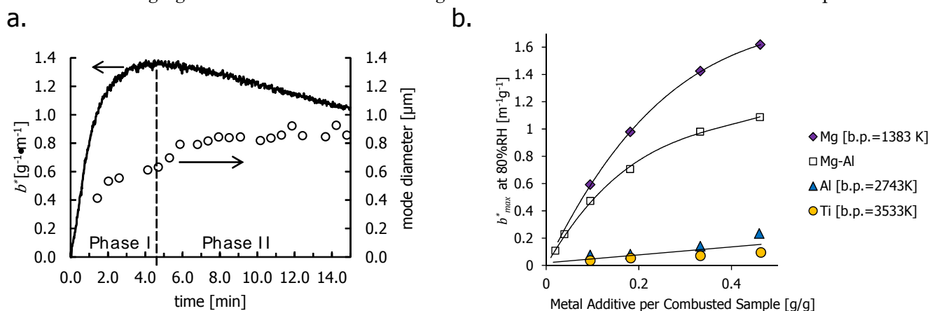
Figure 2. a. Change of sample-mass specific extinction coefficient b^* and mode diameter of aerosol from AP/HTPB composites with 10% CuO additive over time b. Dependence of maximum sample-mass specific extinction coefficient b^*_{max} at 80%RH on amount of metal additive added to the base composition.
