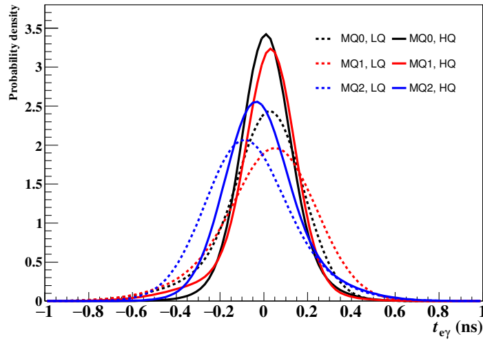
Figure 7.3: t_{ey} PDF of individual 6 categories for 2012 data. HQ and LQ show high and low quality of positron track fitting. MQ means matching quality between DCH and TIC, and (MQ0, MQ1, MQ2) means (good, middle, bad) matching.
