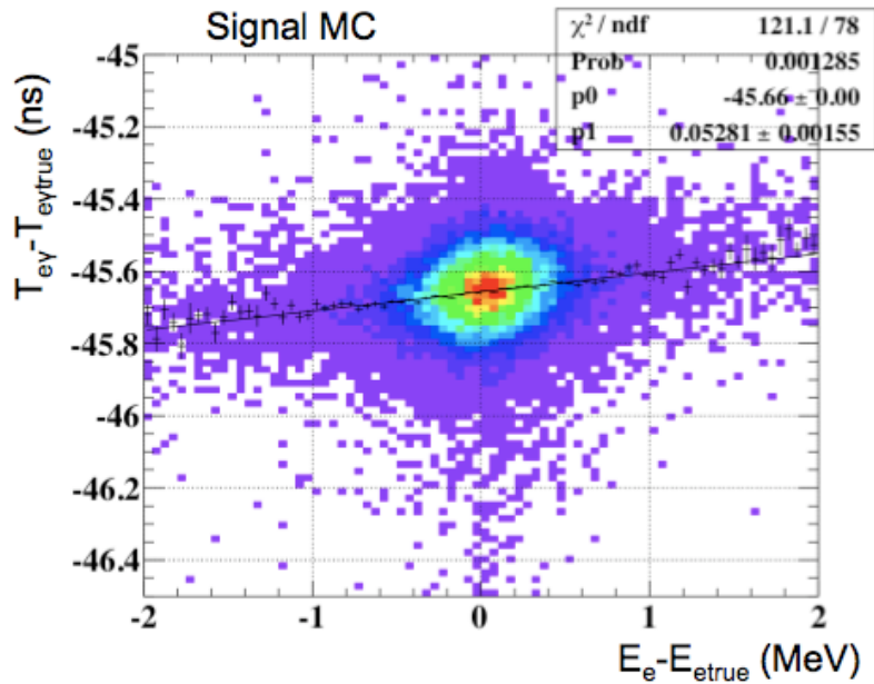
Figure 7.4: The correlation in E_e and t_{ey} for MC signal events. The correlation parameter is extracted by a linear fit on this distribution.
