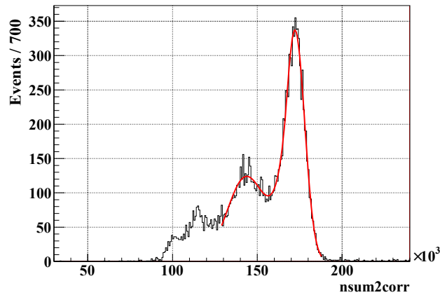
Figure 4.6: An example of the spectrum with {}_{3}^{7}\text{Li}(p, \gamma){}_{4}^{8}\text{Be} reaction. The right most peak is the peak from 17.6 MeV \gamma -ray.
