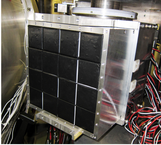
(a) Tagging detector with BGO crystal is installed in detector mover. A cover in front of the crystals is not attached.
