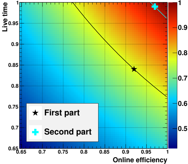
Figure 5.8: Trigger (online) efficiency and livetime ratio in previous scheme (black star) and current scheme (blue cross).
