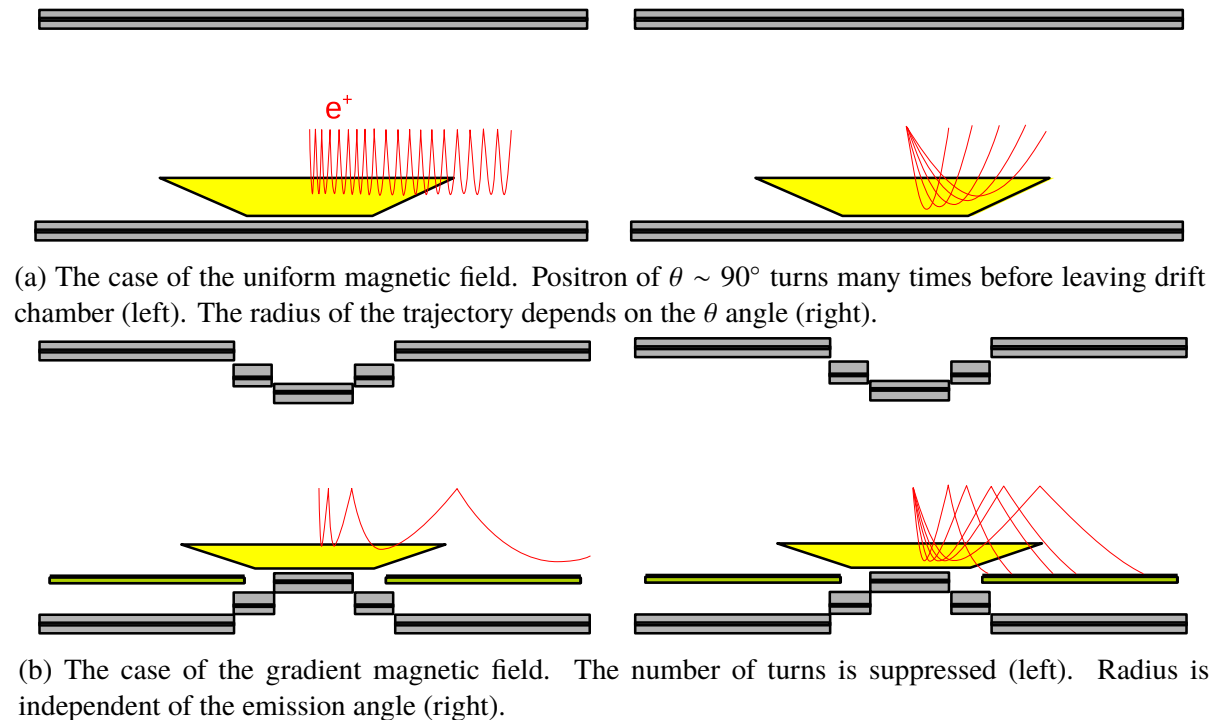
Figure 2.17: Comparison of uniform and gradient field.
