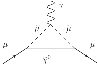
Figure 1.9: An example of contribution to vertex function of \mu in the SUSY model.
