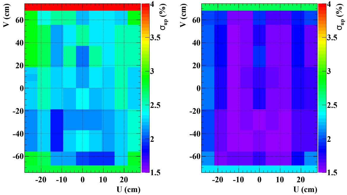
Figure 5.4: Energy resolutions measured in \pi^0 calibration of year 2012. Left and right figures show shallow ( 0 < w < 2 cm) and deep ( w > 2 cm) event, respectively.
