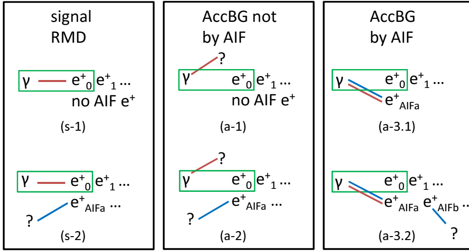
Figure B.1: Types of the events, categorized by the AIF positron. The red line shows the \gamma -ray and its source, the blue line shows the found AIF and the \gamma -ray, and the green box shows the triggered gamma positron pair.
