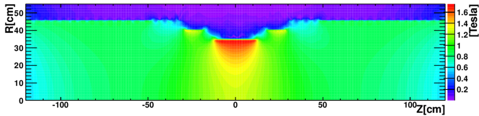
Figure 2.16: Magnetic field by COBRA magnet
