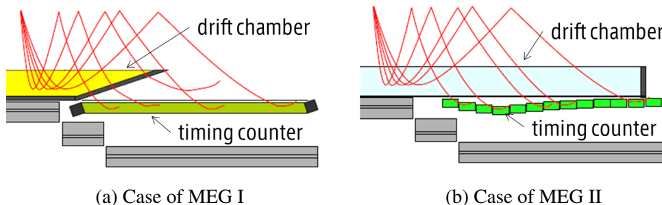
Figure 9.3: Drift chamber is replaced with longer one. The ratio of positrons which is scattered by the support structure will be reduced.
