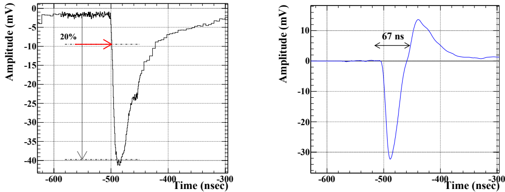
(a) Raw waveform. The horizontal line shows the threshold for timing reconstruction.
