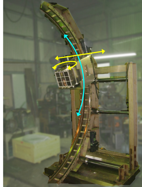
(b) Detector mover, NaI detector is mounted on it. The degree of freedom is shown with arrows.
