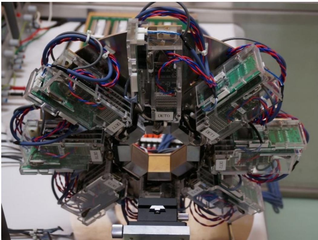
Figure 1. The 8 modules prototype of the small PET system with individual coupling.
