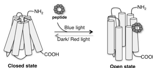
Figure 2. Schematic presentation of the aim of the study. The aim of study is to use peptide to trap the open state of channelrhodopsin (ChR).
