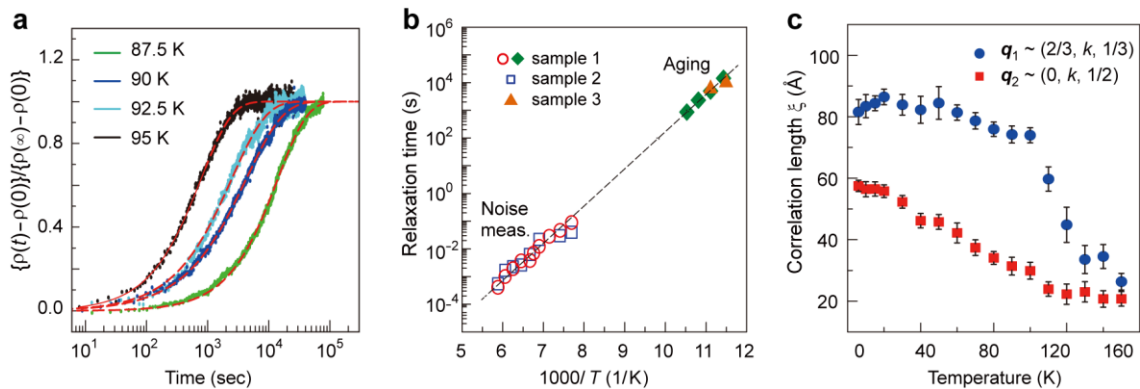
Fig. 2 (a) Physical aging below T_g . (b) 1/T -relaxation time profile. (c) T -dependence of CO domains.
