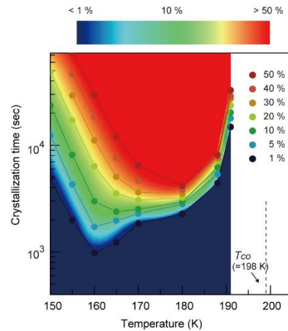
Fig. 3 T-T-T curve in electronic crystal growth.
