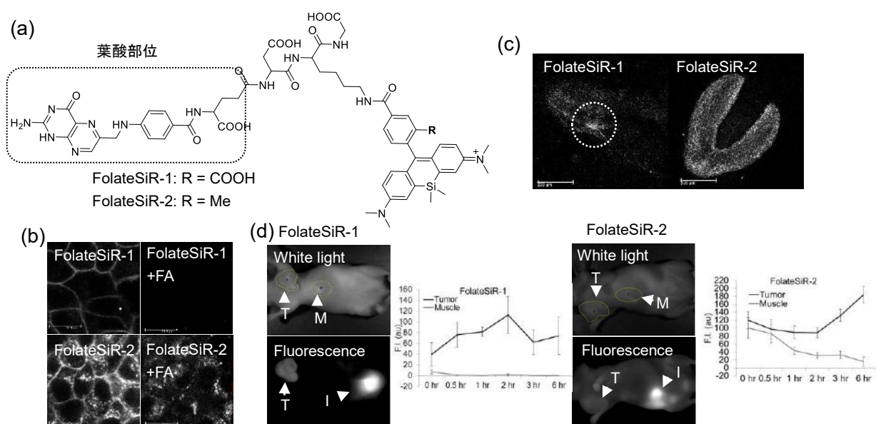
Figure 4. (a) Molecular design of Si-rhodamine-based fluorescent probes for folate receptors. (b) Fluorescence images of KB cells incubated with 5 \mu M FolateSiR-1 or FolateSiR-2 in the presence or absence of 1 mM folic acid (FA) for 30 min at 37 ^{\circ} C. Ex./Em. = 650/670-750 nm. Scale bars: 20 \mu m. (c) Fluorescence images of 8.5-day mouse embryos incubated with 20 \mu M FolateSiR-1 or FolateSiR-2 for 30 min. It is reported that folate receptors are expressed at the neuronal tube closing area (white circle). Scale bars: 200 \mu m. (d) In vivo imaging of KB tumor-bearing mice injected with 100 \mu M FolateSiR-1 in 100 \mu L saline or 100 \mu M FolateSiR-2 in 100 \mu L saline (n = 3). Images were obtained at 30 min after probe loading. Ex./Em. = 661/700-800 nm. T: Tumor; M: Muscle; I: Intestine.
