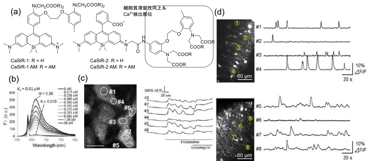
Figure 3. (a) Chemical structures of CaSiR-1 and CaSiR-2. (b) Fluorescence spectra of CaSiR-2 in the presence of various concentrations of Ca 2+ in 30 mM 3-( N -morpholino)propanesulfonic acid (MOPS) buffer containing 100 mM KCl and 10 mM ethylene glycol tetraacetic acid (EGTA), pH 7.2. Ex. 635 nm. (c) Fluorescence images of HeLa cells incubated with 3 μM CaSiR-2 AM for 30 min at 37 °C. Cells were stimulated with 1 μM histamine at 90 sec and 5 μM ionomycin at 210 sec. Ex./Em. = 635/660-750 nm. Scale bars: 20 μm. (d) Fluorescence images of mouse brain slice incubated with 5 μM CaSiR-2 AM (top) and 5 μM CaSiR-1 AM (bottom) for 30 min.
