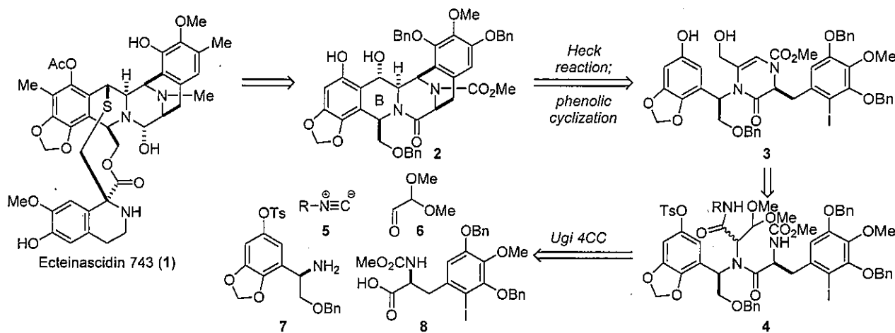
Scheme 1. Synthetic plan of ET-743 (1)
