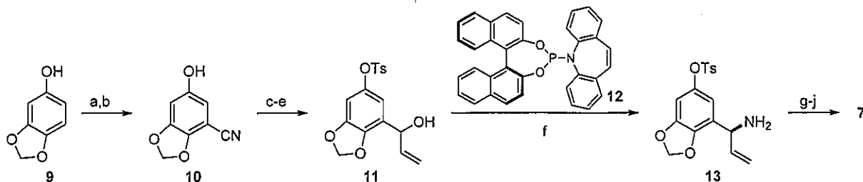
Scheme 2. Preparation of asymmetric amine 7
