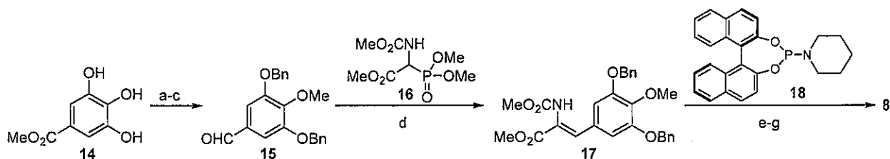
Scheme 3. Preparation of carboxylic acid 8
