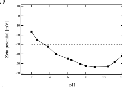
Fig. 1. Zeta potential of GO in buffer solutions of wide pH range
