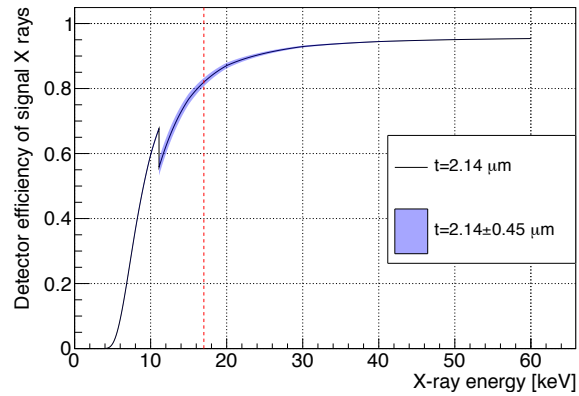
Figure 3.20: The detection efficiency of signal X rays. The uncertainty due to the thickness of the insensitive layer ( 1\sigma ) is also shown by the blue area.
