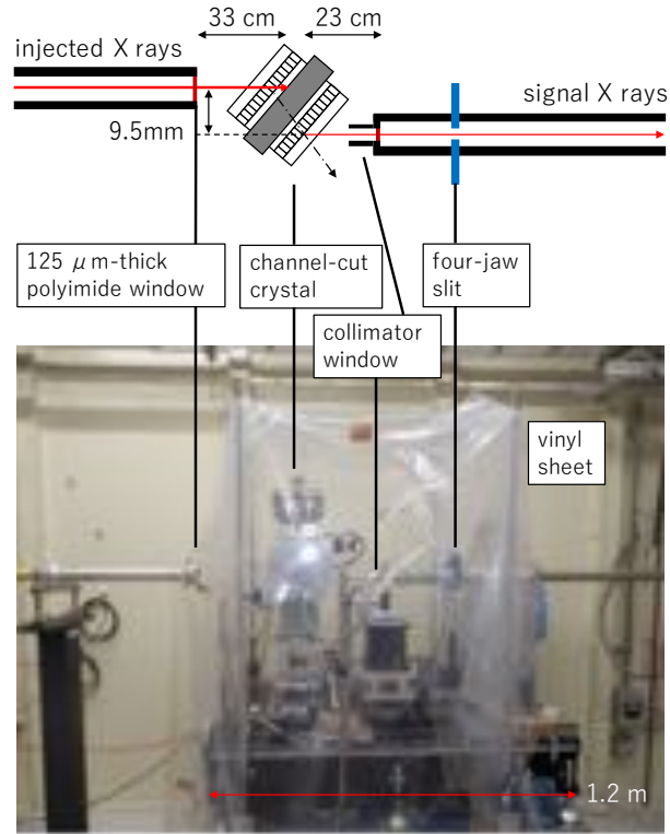
Figure 3.10: The conversion-reconversion system. The system is installed into EH1 of BL19LXU. Upper: schematics of the system. Lower: a picture of the system.
