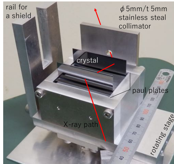
Figure 3.12: The rotating stage.
