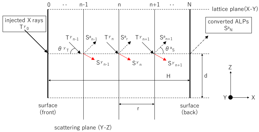
Figure A.6: The X ray-ALP conversion under the Bragg condition of other lattice planes. X-ray diffraction takes place on a plane other than the X - Z plane. See also Fig. A.4.
