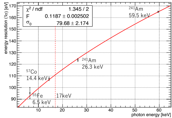
Figure 3.17: The energy resolution of the germanium detector. Data points show the energy resolution ( 1\sigma ) measured by using checking sources ( ^{241}\text{Am} , ^{57}\text{Co} and ^{55}\text{Fe} ).
