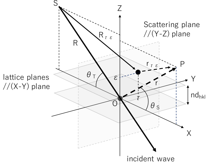
Figure A.3: Schematics of the conversion by a virtual scattering plane. The lattice planes of the crystal is parallel to the X-Y plane, the conversion occurs on the X-Z plane and scattering planes are parallel to the Y-Z plane and crystal surfaces. X rays are assumed to be \sigma -polarized.
