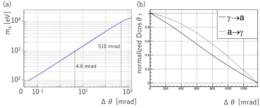
Figure 2.5: The \Delta\theta dependence of resonant ALPs' mass and relative sensitivity to g_{a\gamma\gamma} . (a): the resonant mass. The same condition as Fig. 2.4 is assumed. The upper limit of \Delta\theta corresponds to \theta_T^\gamma = 90 deg. (b) the factor, D\cos\theta_T , normalized by its maximum value of \cos\theta_T ( \Delta\theta = 0 ). The normalized value corresponds to the relative sensitivity to g_{a\gamma\gamma} .
