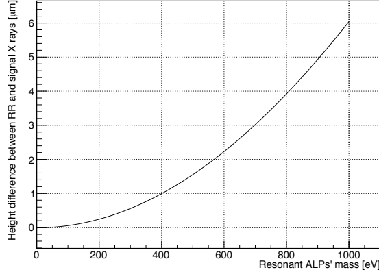
Figure 3.24: The height difference between RR beams and reconverted X rays as a function of the resonant ALPs' mass.
