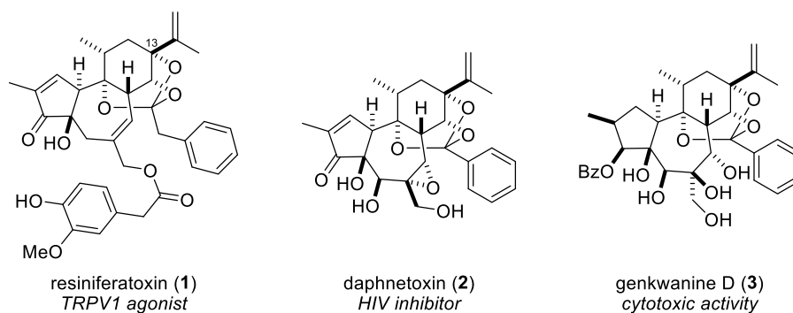
Figure 1. Daphnane diterpenoids
