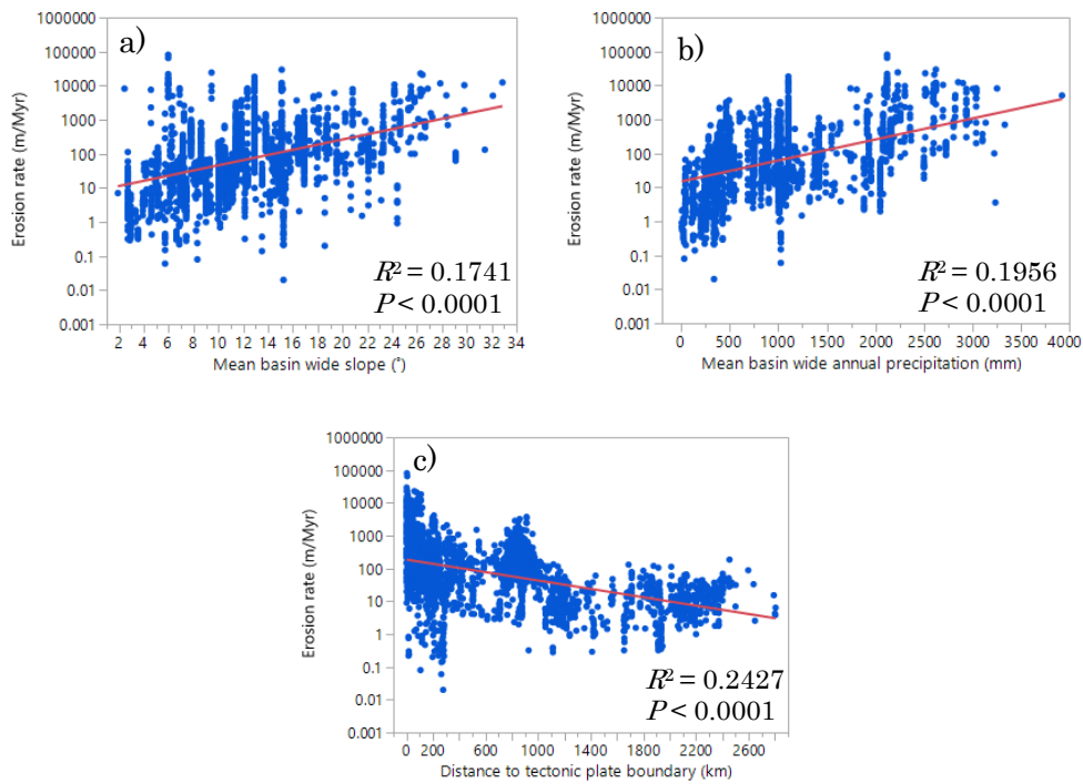
Figure 2. Erosion rates as a function of key parameters: a) Mean basin-wide slope; b) Mean annual basin-wide precipitation; and c) Distance to tectonic plate boundary.
