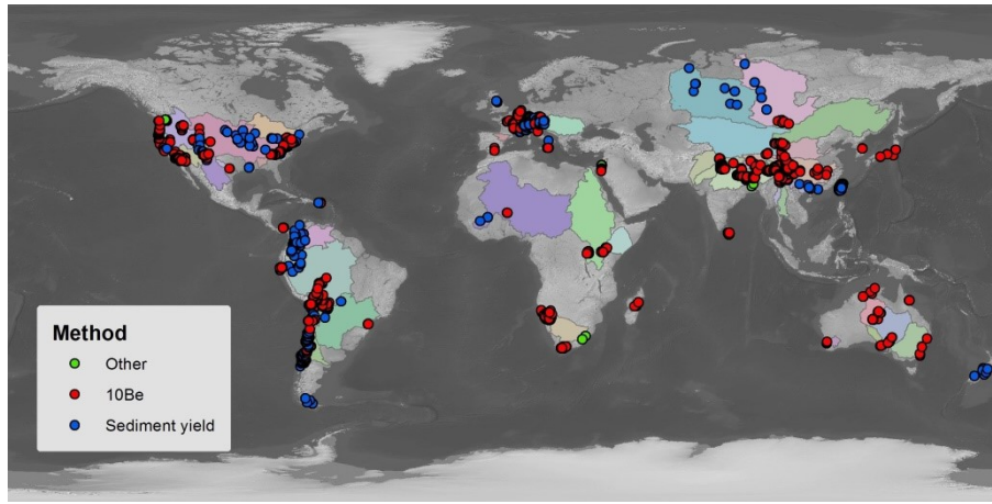
Figure 1. Data location and type map. All the data originate from previously published papers or were downloaded as sediment yield data from the U.S. Geological Survey data portal website. Most of the erosion rates were derived from either sediment yield or from cosmogenic ^{10}\text{Be} however, other methods such as ^{36}\text{Cl} or fission tracks were included in the compilation.
