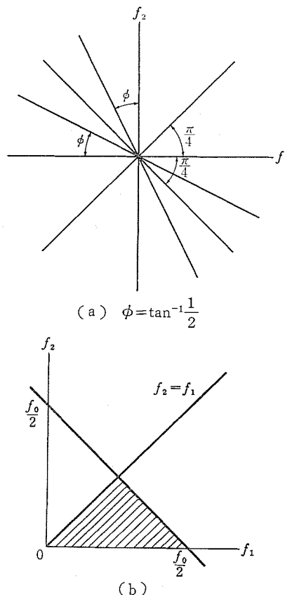
第1図 バイスペクトルの推定領域 Fig. 1 (a) The bispectrum b(f_1, f_2) is completely specified by its values in any one of the twelve sectors. (b) The oblique lines indicate the area where the bispectrum is estimated when the sampling theorem is taken into account.
