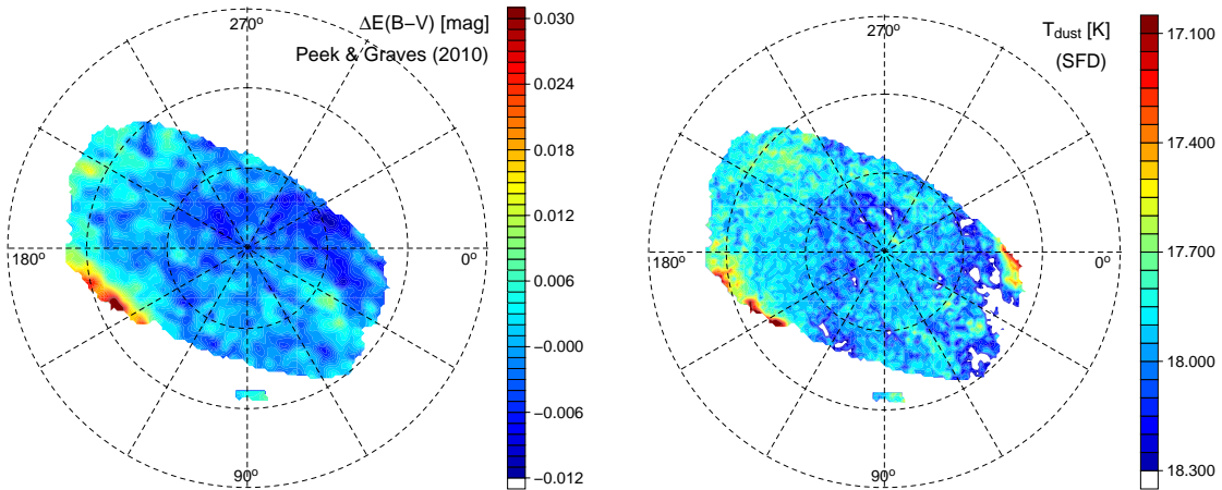
Figure 3.5: Left panel ; Correction to the SFD map in E(B - V) provided by Peek & Graves (2010) at the resolution of \sim 4''.5 . This correction term, \Delta E(B - V) , is to be added to the SFD map extinction. The projection is the same as Figure 3.3, but the data are only available for the SDSS sky area in the north galactic hemisphere. Right panel ; Dust temperature map by SFD as the same as Figure 3.3, but only the SDSS sky area is shown for visual comparison with left panel .
