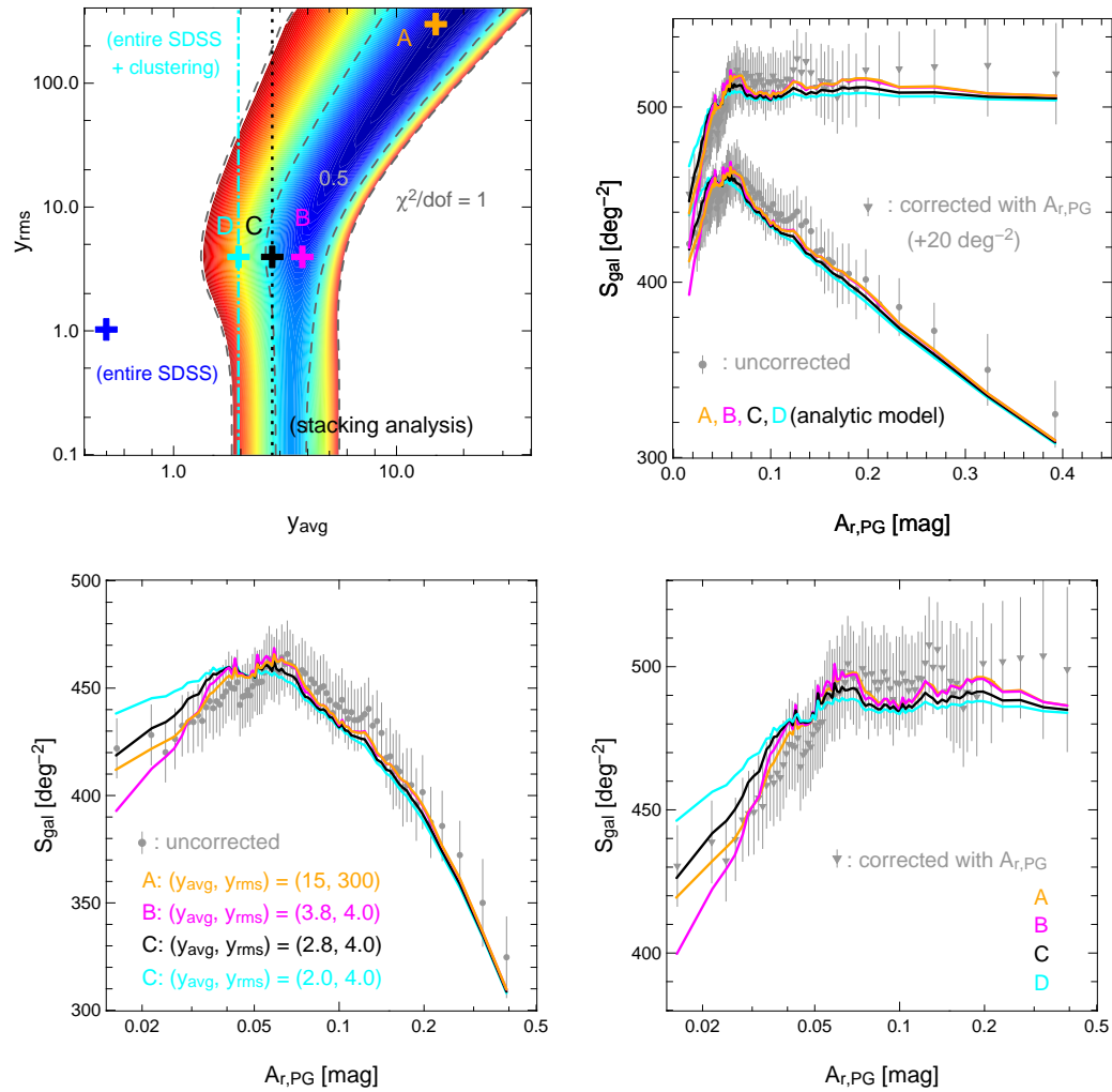
Figure 5.15: Fit to the observed anomaly using the analytical model, as the same as Figure 5.12, but for the corrected extinction map provided by Peek & Graves (2010), A_{r,\text{PG}} . The reference values of y_{\text{avg}} and y_{\text{rms}} indicated as crosses are the same as Figure 5.12.
