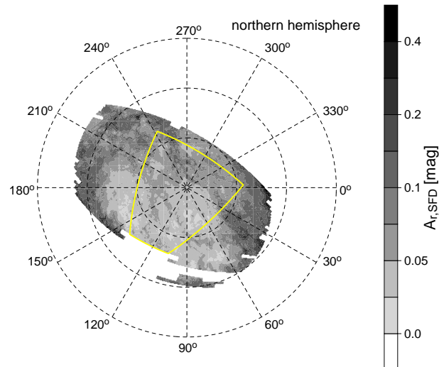
Figure 4.1: The region of the sky used for the present analysis, which is shaded according to the extinction value A_{r,\text{SFD}} . The yellow lines indicate the inner regions used for comparison in Subsection 4.2.2.
