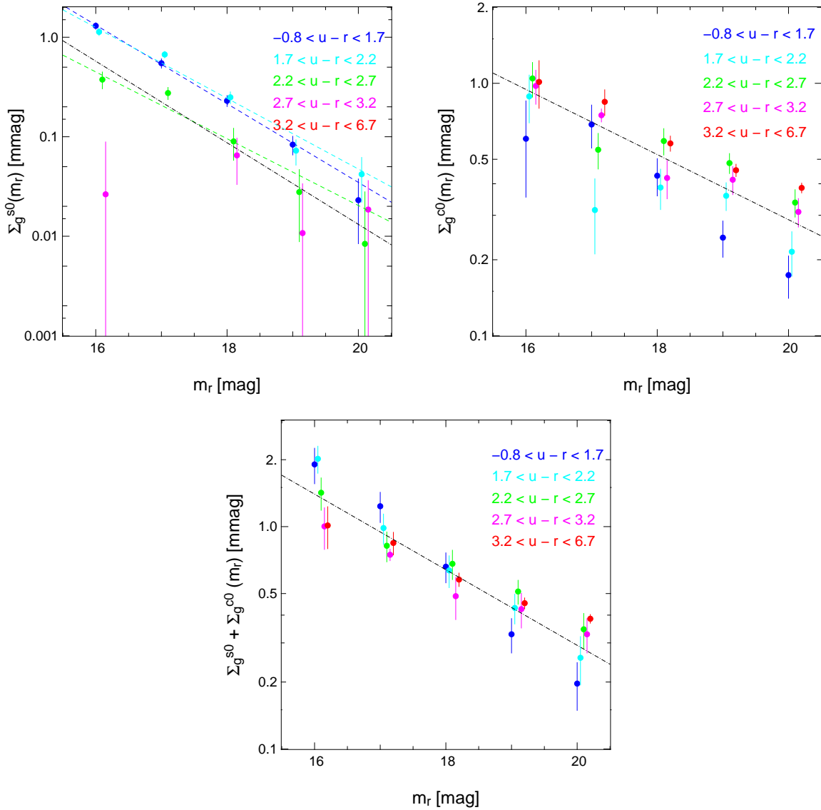
Figure 5.20: The best-fit values of \Sigma_g^{s0} (top left), \Sigma_g^{c0} (top right), and \Sigma_g^{s0} + \Sigma_g^{c0} (bottom) for m_r and u - r binned 25 subsamples. Blue, cyan, green, magenta, and red symbols indicate the best-fit values for -0.8 < u - r < 1.7 , 1.7 < u - r < 2.2 , 2.2 < u - r < 2.7 , 2.7 < u - r < 3.2 , and 3.2 < u - r < 6.7 , respectively. The error bars are computed from 400 jackknife resampling. Dashed lines in the top left panel indicate the best-fit power law of equation (5.29), for -0.8 < u - r < 1.7 , 1.7 < u - r < 2.2 , and 2.2 < u - r < 2.7 . Dot-dashed (black) lines in each panel indicate the best-fit power law for the entire sample, neglecting the color dependence shown Figure 4.11. The best-fit values of \Sigma_g^{s0} for 3.2 < u - r < 6.7 are zero for all m_r bin, therefore not shown here.
