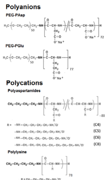
Figure 1: Block polyanion and homo polycation polymers used in PIC preparation
