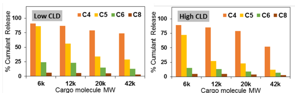
Figure 4. Release amounts of cargo molecules from PICsomes with different polycation side chain lengths at 37°C
