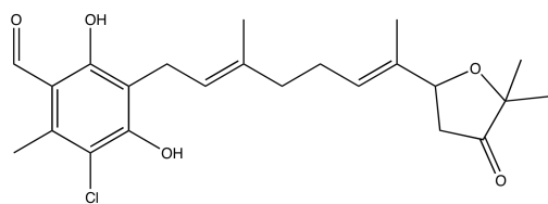
(Figure 1) Ascofuranone
